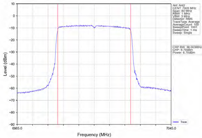
802.11ax(HEW40)_MCH_7005MHz_RU484_Left_Ant2_NTNV
