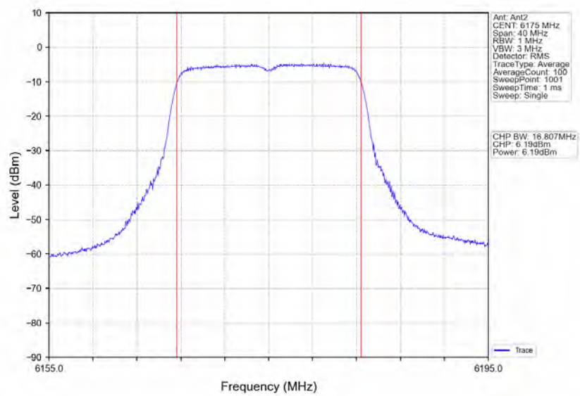
802.11a_MCH_6175MHz_Ant2_NTNV
