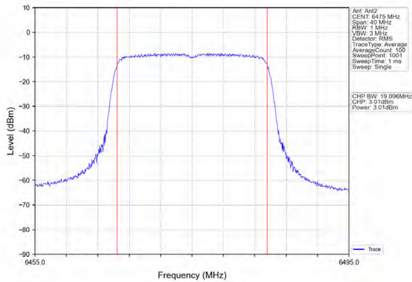
802.11ax(HEW20)_MCH_6475MHz_RU242_Left_Ant2_NTNV
