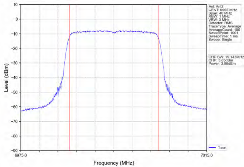
802.11ax(HEW20)_MCH_6995MHz_RU242_Left_Ant2_NTNV
