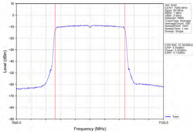
802.11ax(HEW40)_HCH_7085MHz_RU484_Left_Ant2_NTNV
