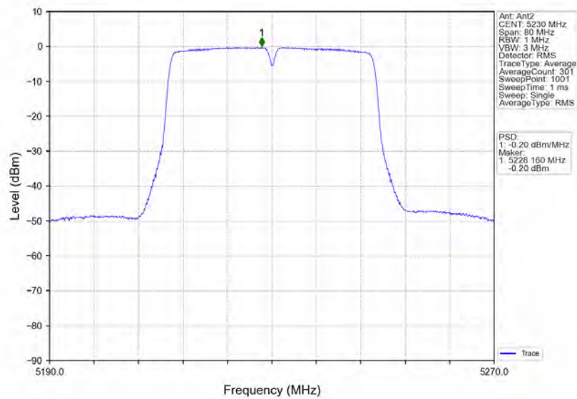
802.11n(HT40)_HCH_5230MHz_MIMO_NTNV
