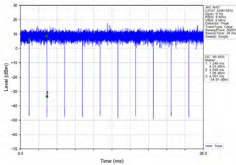
802.11ac(VHT80)_MCH_5290MHz_Ant1_NTNV
