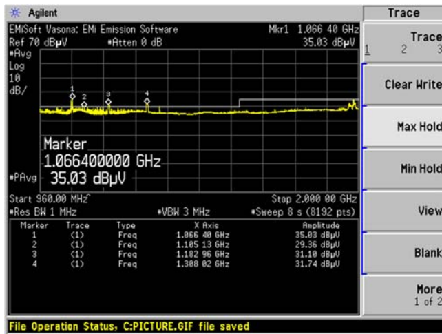
960 MHz-2 GHz H-Pol
