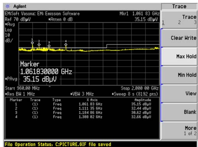
960 MHz-2 GHz V-Pol
