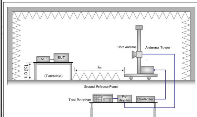
Above 1GHz
