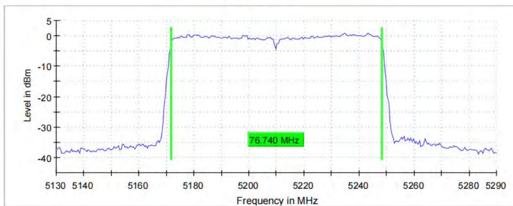
99 % Bandwidth
