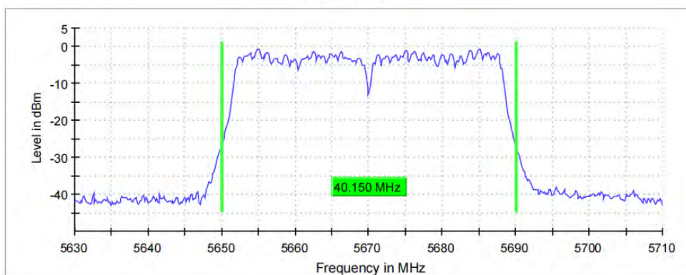
26 dB Bandwidth
