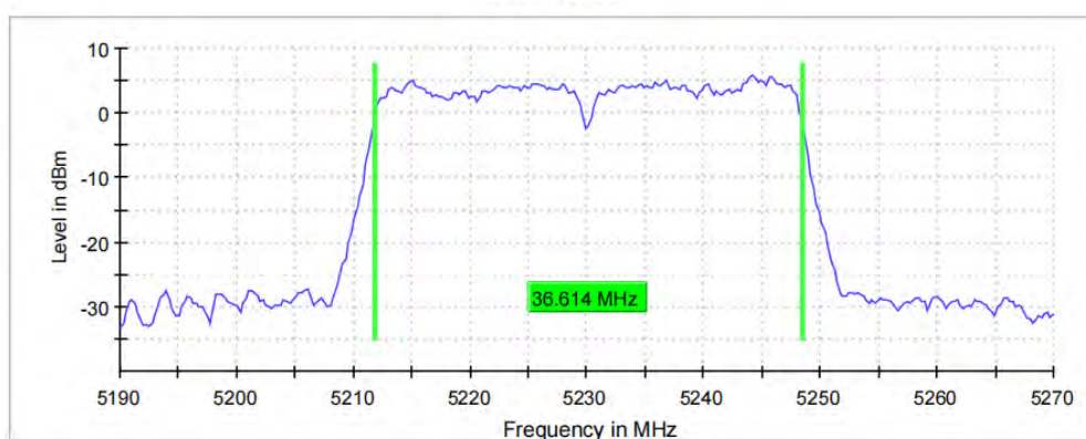
99 % Bandwidth
