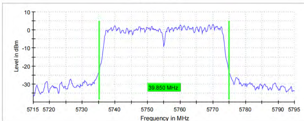
26 dB Bandwidth
