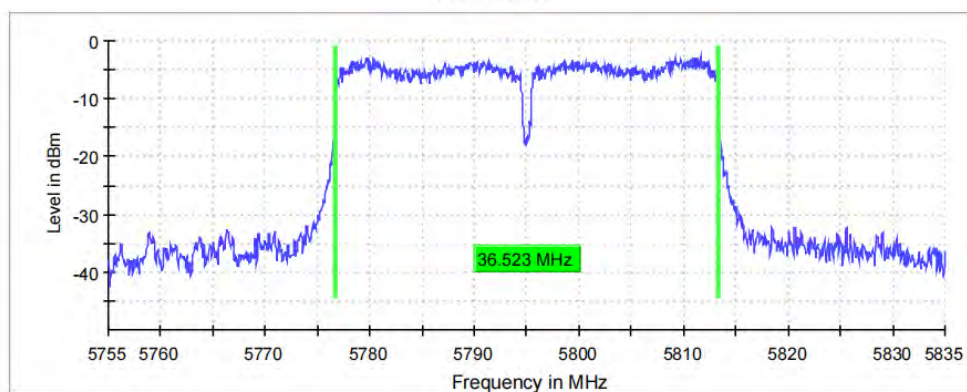
6 dB Bandwidth
