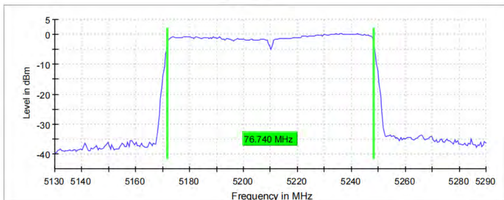
99 % Bandwidth
