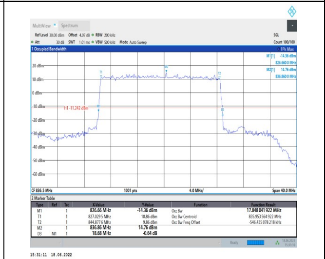
1-N5--15-20-M-2-DFT-PI2BPSK-Outer_Full-100@0-Ant 1-17.848-18.680-≤20-PASS
