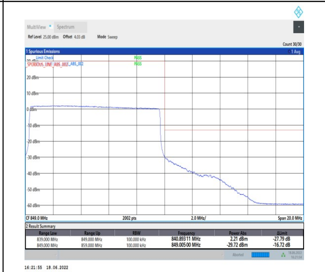
1-N5--15-10-H-6-CP-QPSK-Outer_Full-52@0-Ant1-seegraph-PASS-see graph
