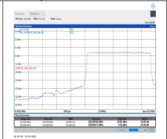
1-N5--15-10-L-3-DFT-PI2BPSK-Outer_Full-50@0-Ant1-seegraph-PASS-see graph
