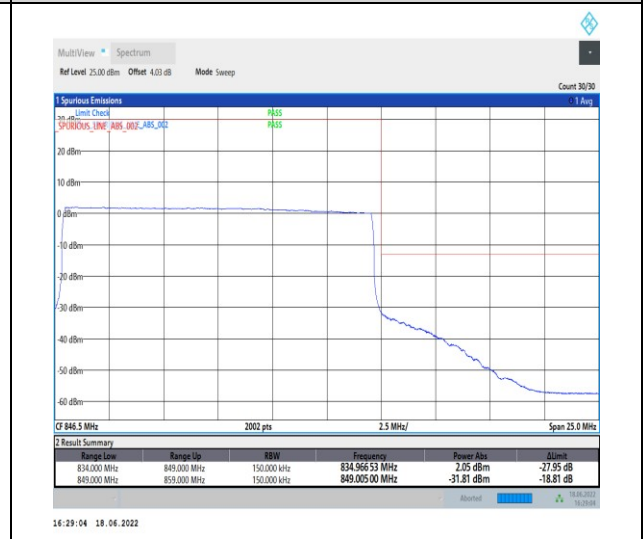
1-N5--15-15-H-6-CP-QPSK-Outer_Full-79@0-Ant1-seegraph-PASS-see graph
