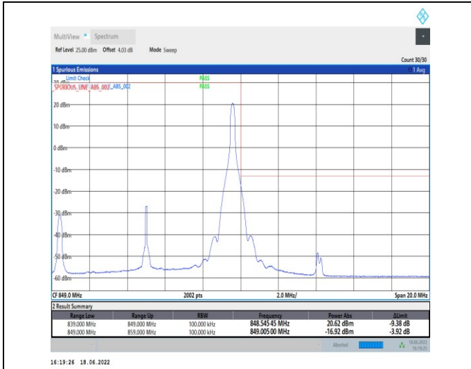
1-N5--15-10-H-2-DFT-PI2BPSK-Edge_1RB_Right-1@51-Ant1-seegraph-PASS-see graph
