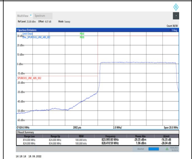
1-N5--15-10-L-6-CP-QPSK-Outer_Full-52@0-Ant1-seegraph-PASS-see graph
