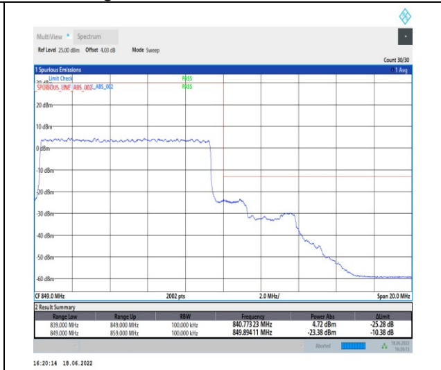
1-N5--15-10-H-3-DFT-PI2BPSK-Outer_Full-50@0-Ant1-seegraph-PASS-see graph
