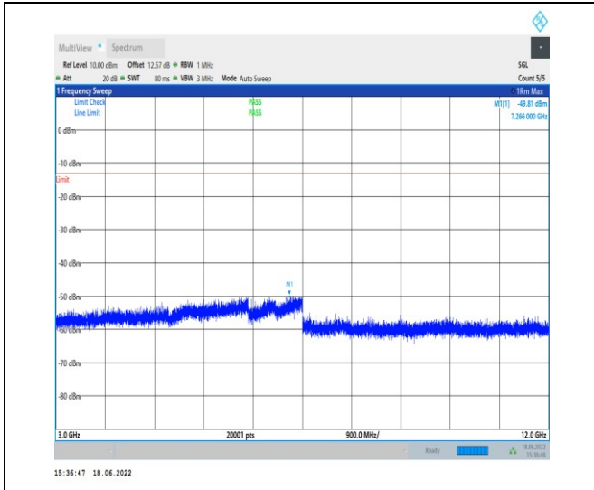
1-N5--15-20-L-1-DFT-PI2BPSK-Inner_1RB_Left-1@ 1-3000-12000-Ant1--49.81--13-PASS
