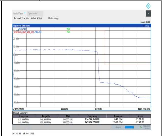
1-N5--15-20-H-3-DFT-PI2BPSK-Outer_Full-100@0-Ant1-seegraph-PASS-see graph
