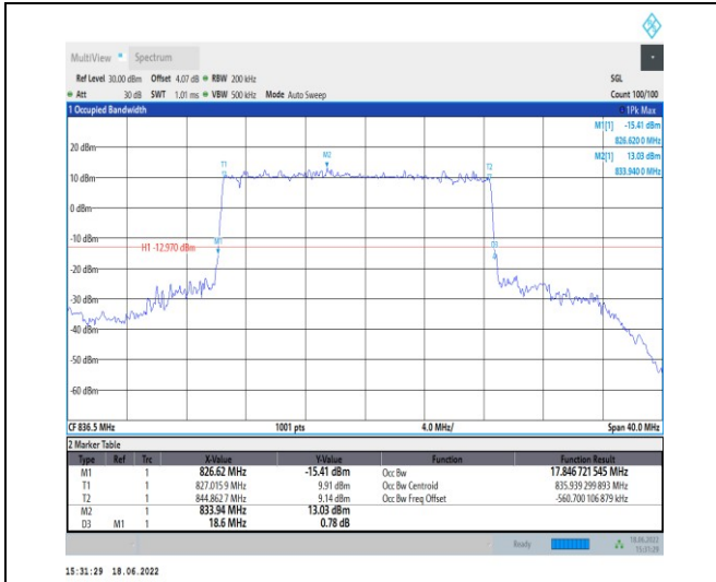
1-N5--15-20-M-3-DFT-16QAM-Outer_Full-100@0-A nt1-17.847-18.600-≤20-PASS
