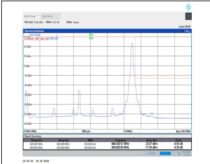
1-N5--15-20-H-2-DFT-PI2BPSK-Edge_1RB_Right-1@105-Ant1-seegraph-PASS-see graph
