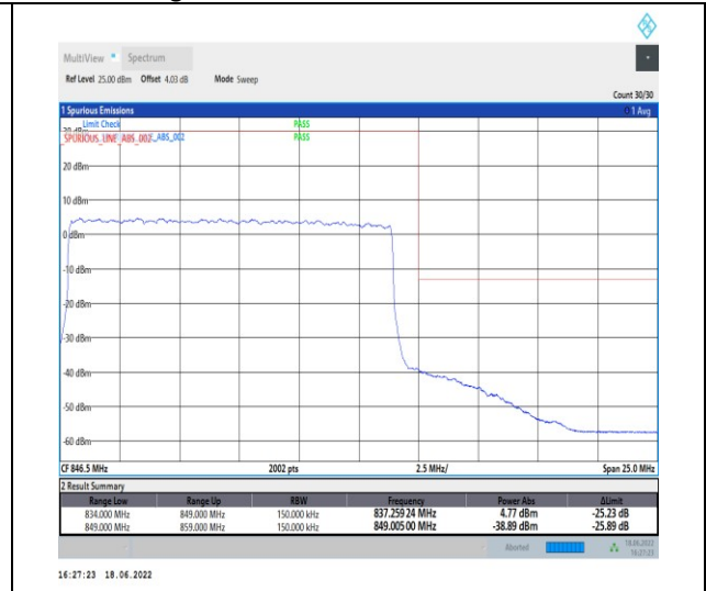
1-N5--15-15-H-3-DFT-PI2BPSK-Outer_Full-75@0-Ant1-seegraph-PASS-see graph
