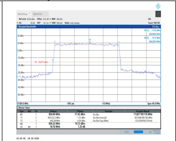
1-N5--15-20-L-5-DFT-256QAM-Outer_Full-100@0-Ant1-17.828-18.760-<=20-PASS
