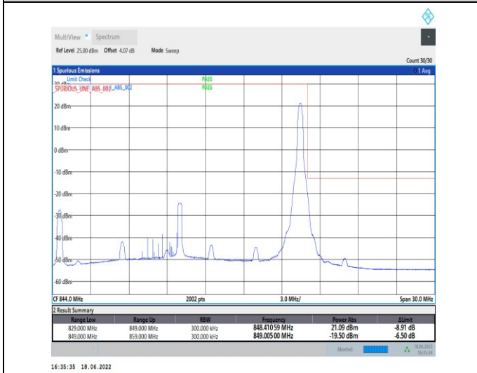
1-N5--15-20-H-5-CP-QPSK-Edge_1RB_Right-1@105-Ant1-seegraph-PASS-see graph
