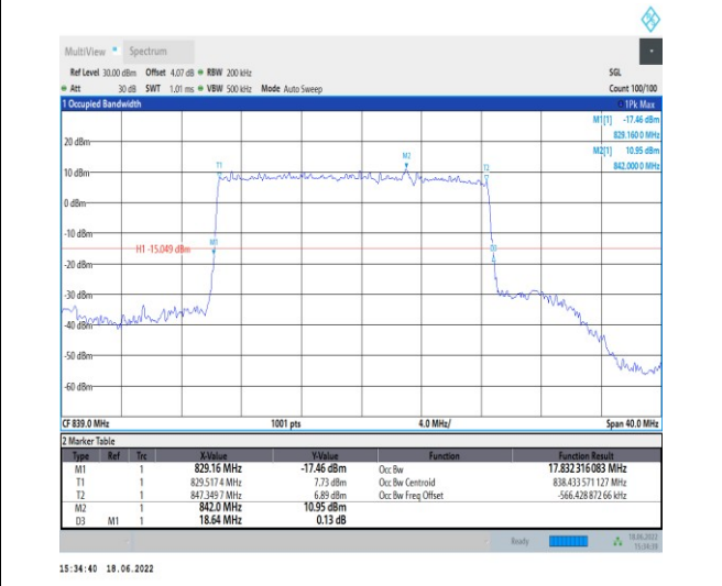
1-N5--15-20-H-5-DFT-256QAM-Outer_Full-100@0-Ant1-17.832-18.640-≤20-PASS
