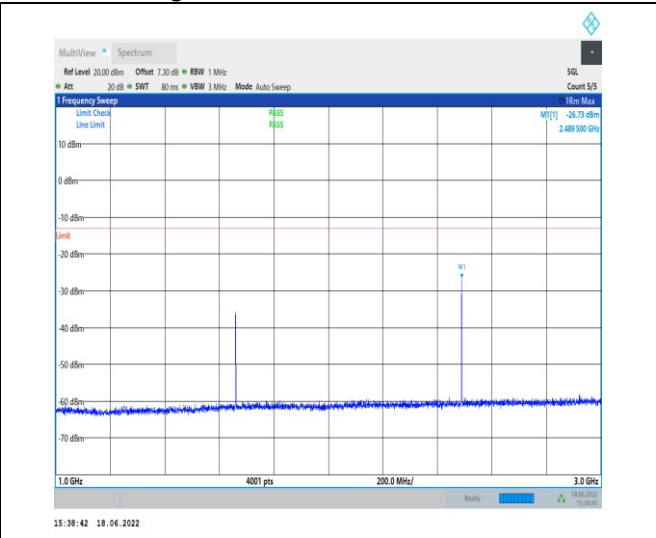
1-N5--15-20-H-1-DFT-PI2BPSK-Inner_1RB_Left-1@ 1-1000-3000-Ant1--26.73--13-PASS
