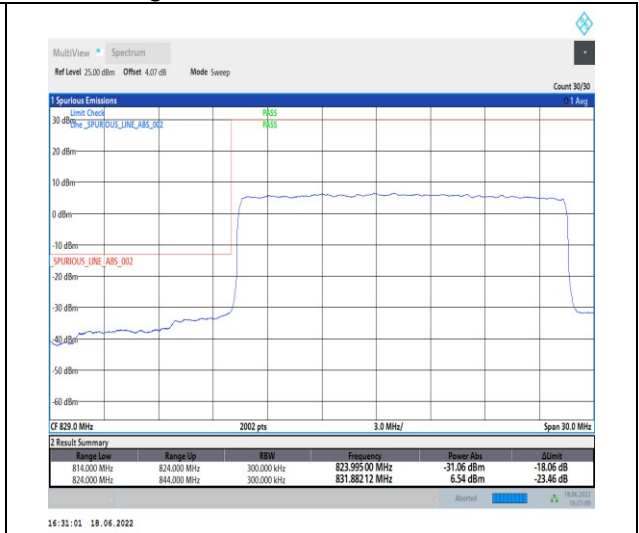
1-N5--15-20-L-3-DFT-PI2BPSK-Outer_Full-100@0-Ant1-seegraph-PASS-see graph
