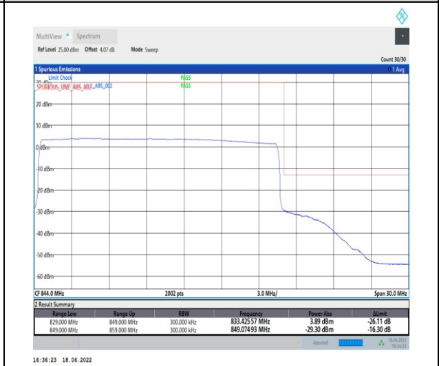
1-N5--15-20-H-6-CP-QPSK-Outer_Full-106@0-Ant1-seegraph-PASS-see graph
