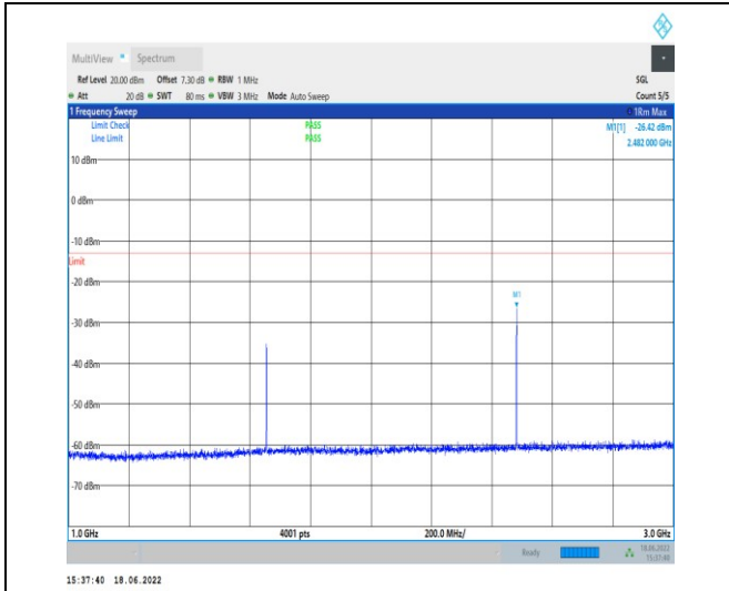
1-N5--15-20-M-1-DFT-PI2BPSK-Inner_1RB_Left-1@ 1-1000-3000-Ant1--26.42--13-PASS
