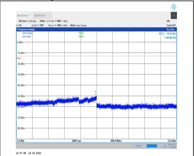
1-N5--15-20-M-1-DFT-PI2BPSK-Inner_1RB_Left-1@ 1-3000-12000-Ant1--49.25--13-PASS
