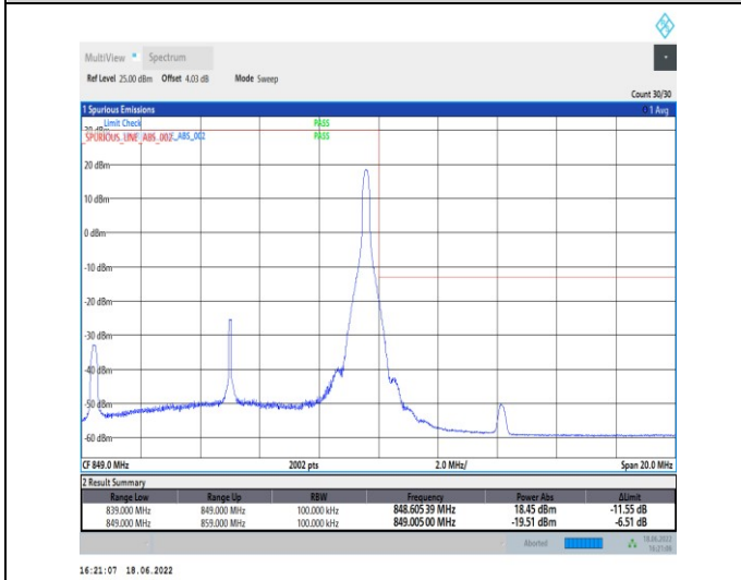
1-N5--15-10-H-5-CP-QPSK-Edge_1RB_Right-1@51-Ant1-seegraph-PASS-see graph
