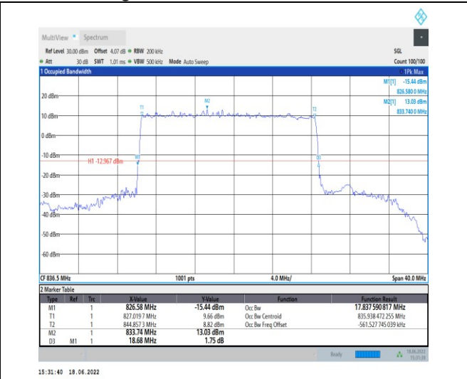
1-N5--15-20-M-4-DFT-64QAM-Outer_Full-100@0-A nt1-17.838-18.680-≤20-PASS
