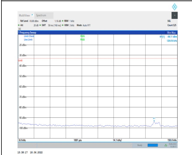
1-N5--15-20-H-1-DFT-PI2BPSK-Inner_1RB_Left-1@ 1-0.009-0.15-Ant1--94.11--33-PASS
