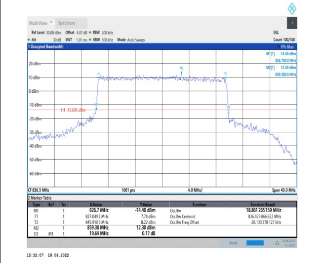
1-N5--15-20-M-6-CP-QPSK-Outer_Full-106@0-A nt1-18.861-19.640-≤20-PASS
