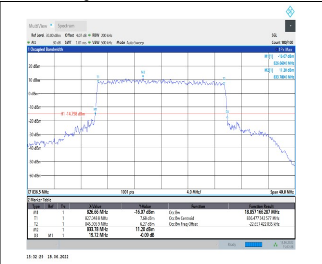
1-N5--15-20-M-8-CP-64QAM-Outer_Full-106@0-Ant 1-18.857-19.720-≤20-PASS
