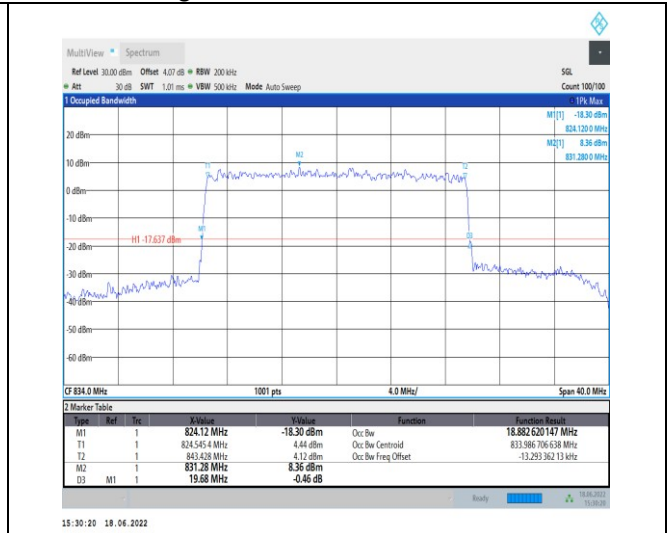
1-N5--15-20-L-9-CP-256QAM-Outer_Full-106@0-Ant 1-18.883-19.680-≤20-PASS
