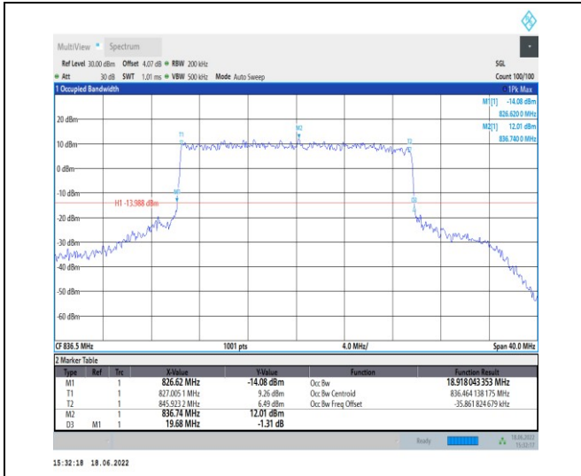
1-N5--15-20-M-7-CP-16QAM-Outer_Full-106@0-Ant 1-18.918-19.680-≤20-PASS
