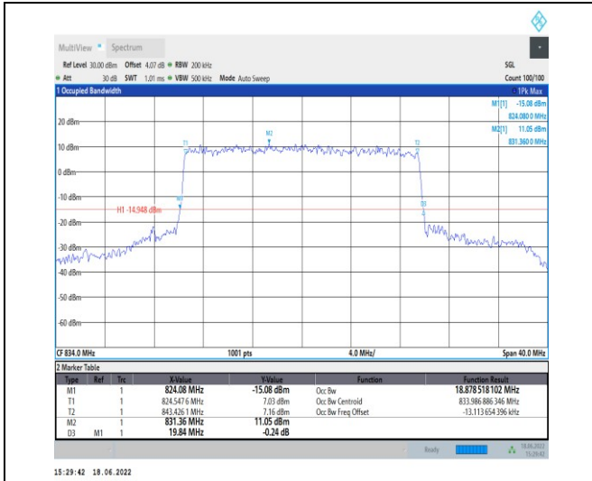
1-N5--15-20-L-8-CP-64QAM-Outer_Full-106@0-Ant 1-18.879-19.840-≤20-PASS
