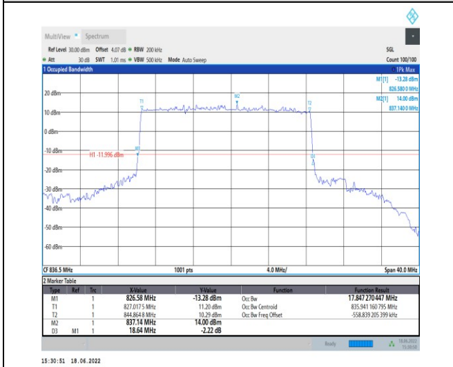
1-N5--15-20-M-1-DFT-QPSK-Outer_Full-100@0-Ant 1-17.847-18.640-≤20-PASS
