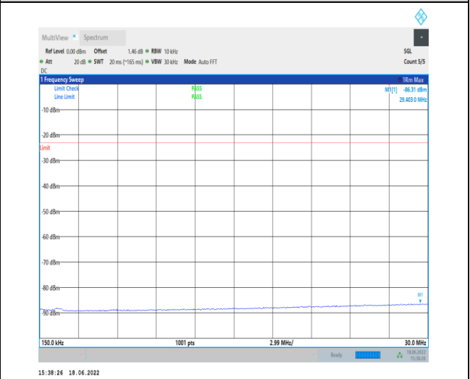
1-N5--15-20-H-1-DFT-PI2BPSK-Inner_1RB_Left-1@ 1-0.15-30-Ant1--86.31--23-PASS
