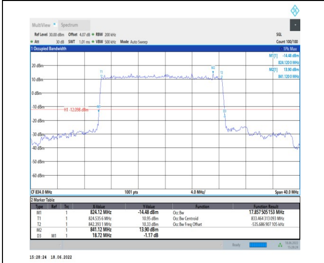
1-N5--15-20-L-2-DFT-PI2BPSK-Outer_Full-100@0-A nt1-17.858-18.720-≤20-PASS
