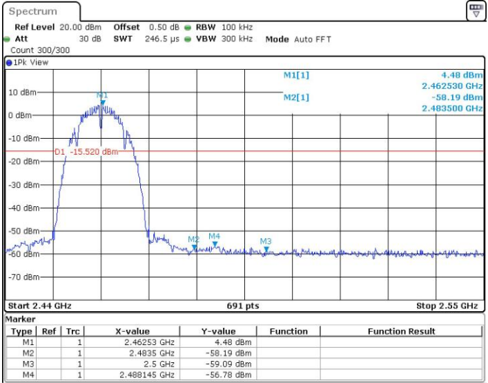
11B_Ant2_High_2462
