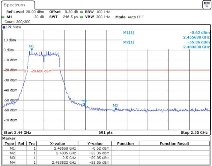
11G_Ant2_High_2462
