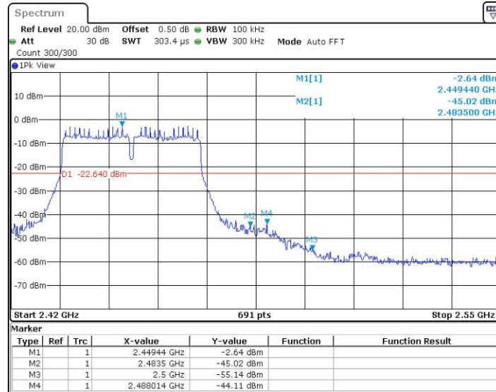
11N40_Ant1_High_2452
