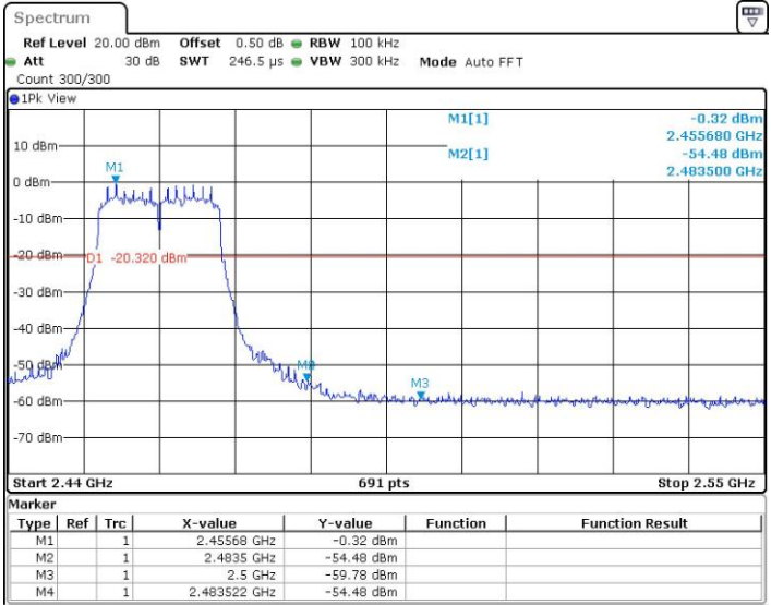
11N20_Ant2_High_2462
