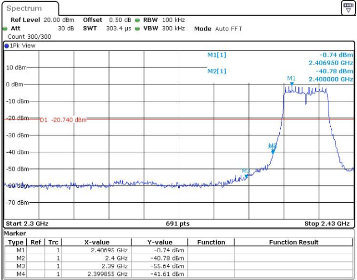
11G_Ant2_Low_2412
