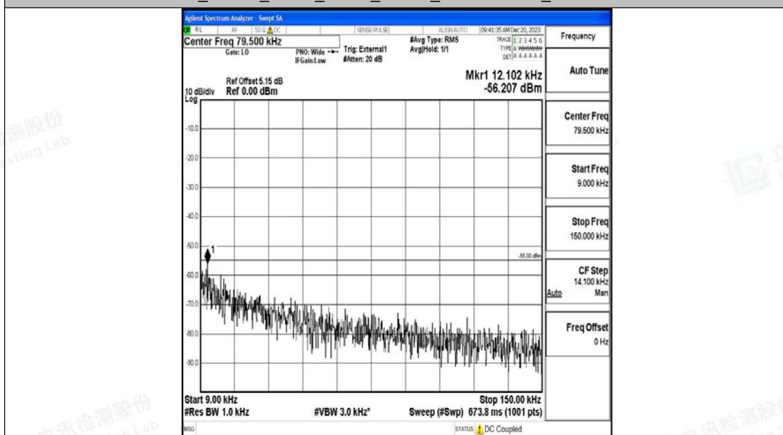
Band41_10MHz_16QAM_40620_1RB#0_0.009~0.15_0.009~0.15
