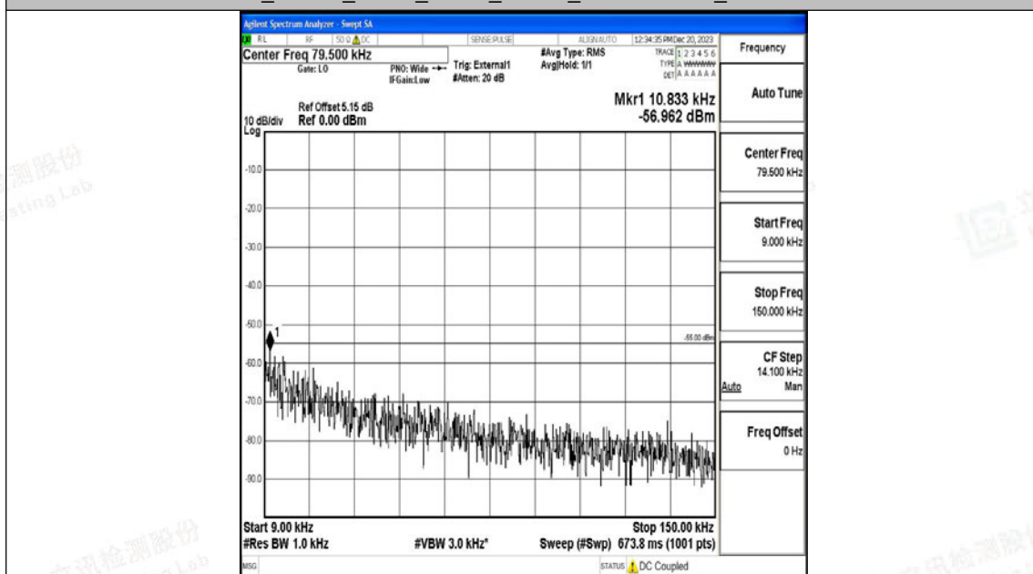
Band38_20MHz_16QAM_37850_1RB#0_0.009~0.15_0.009~0.15
