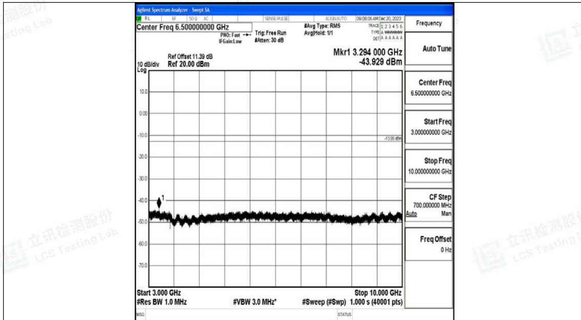
Band26_10MHz_QPSK_26990_1RB#0_3000~10000_3000~10000
