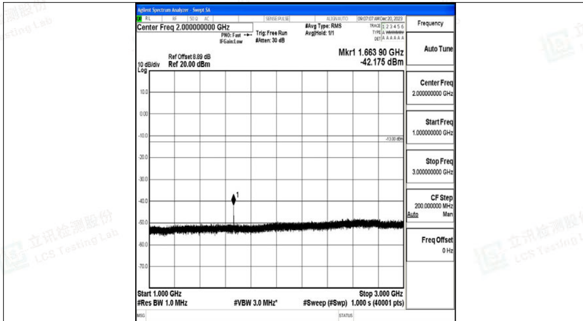
Band26_10MHz_16QAM_26915_1RB#0_1000~3000_1000~3000
