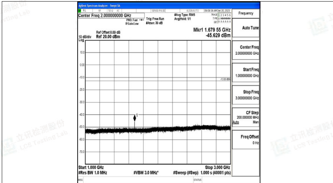
Band26_10MHz_16QAM_26990_1RB#0_1000~3000_1000~3000
