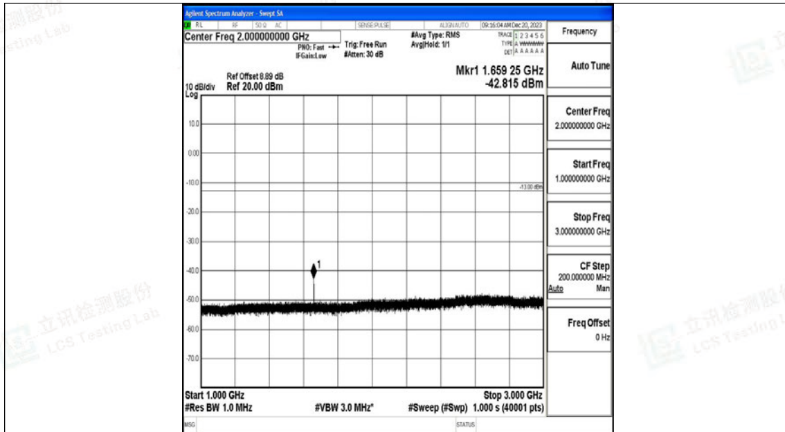
Band26_15MHz_16QAM_26915_1RB#0_1000~3000_1000~3000
