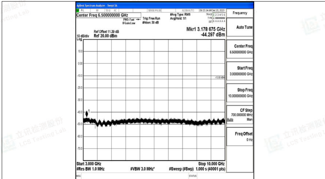
Band26_15MHz_QPSK_26915_1RB#0_3000~10000_3000~10000
