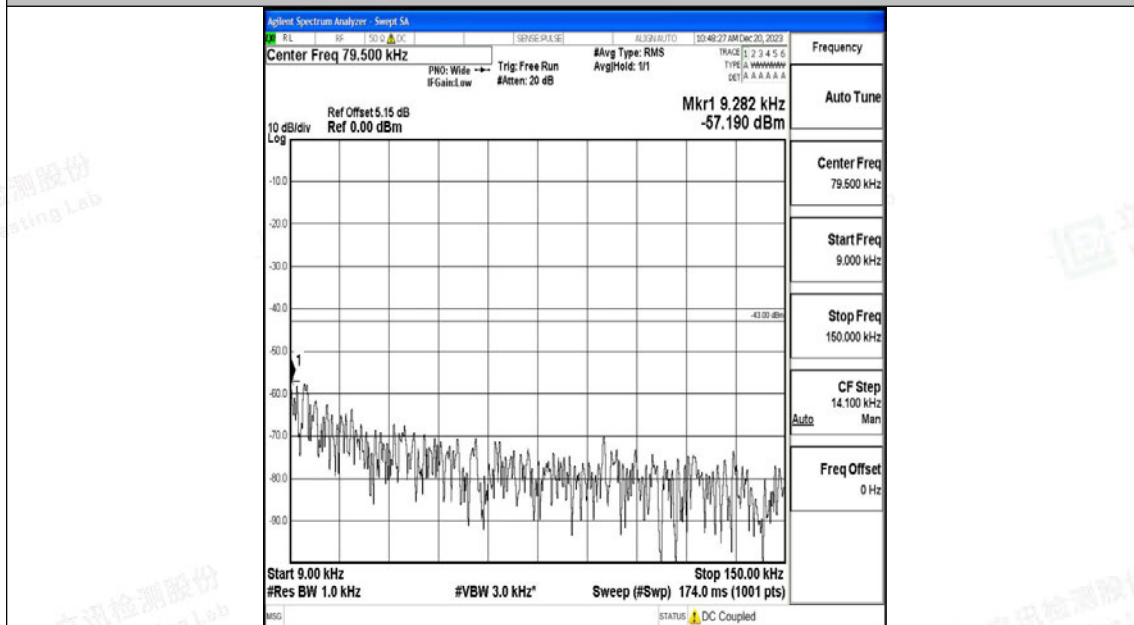
Band25_5MHz_QPSK_26365_1RB#0_0.009~0.15_0.009~0.15
