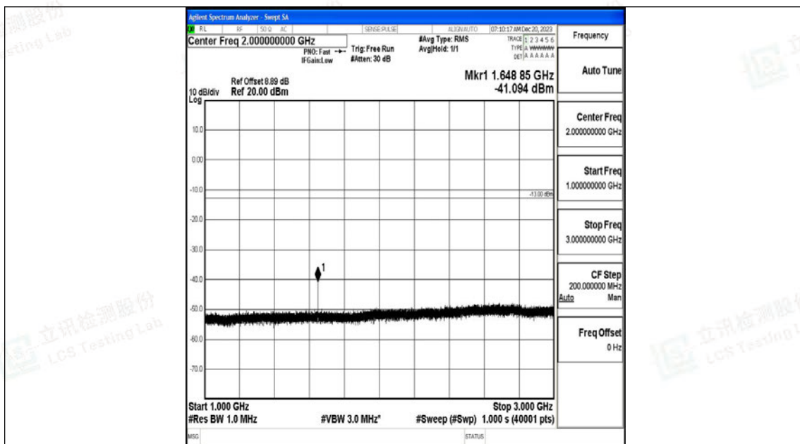
Band5_5MHz_16QAM_20425_1RB#0_1000~3000_1000~3000
