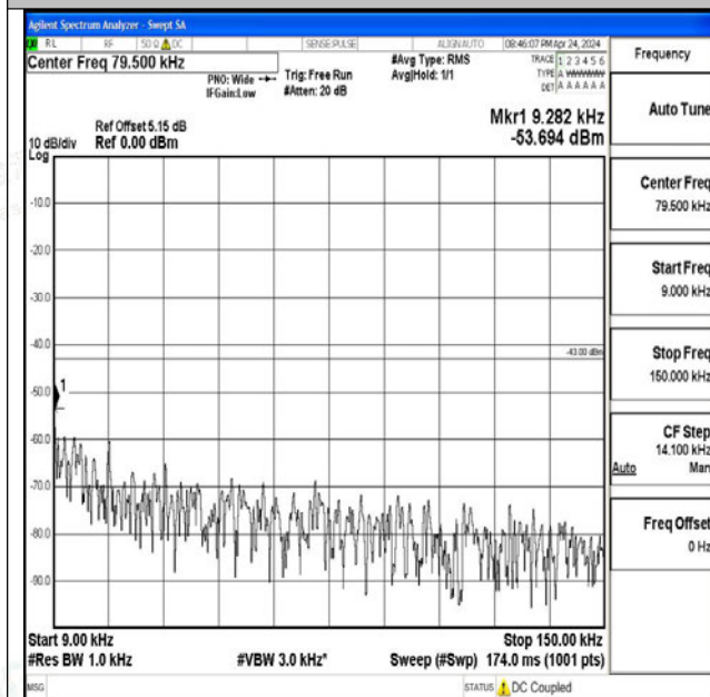
Band66_20MHz_QPSK_132072_1RB#0_0.009~0.15_0.0 09~0.15
