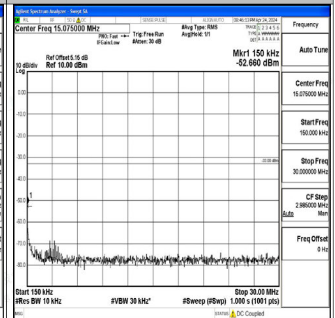
Band66_20MHz_QPSK_132072_1RB#0_0.15~30_0.15~ 30
