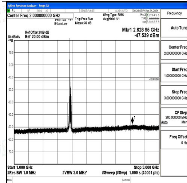
Band66_15MHz_16QAM_132597_1RB#0_1000~3000_1 000~3000
