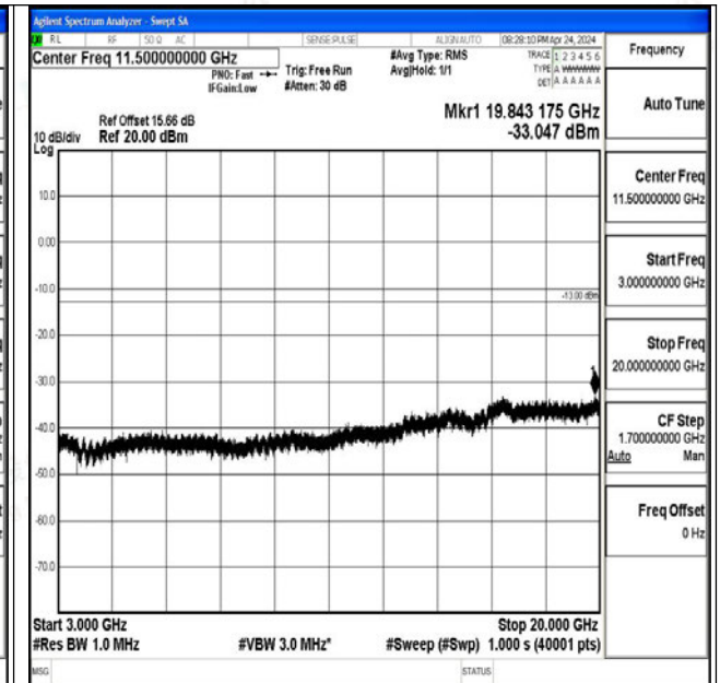
Band66_15MHz_16QAM_132597_1RB#0_3000~20000_ 3000~20000
