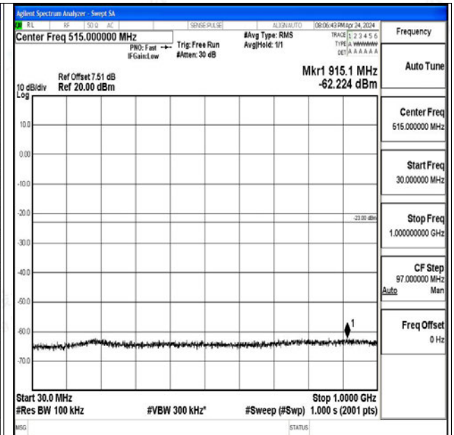
Band66_10MHz_16QAM_132622_1RB#0_30~1000_30~1000 1000
