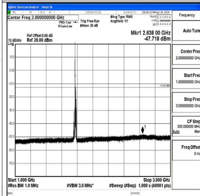
Band66_10MHz_16QAM_132622_1RB#0_1000~3000_1000~3000 000~3000
