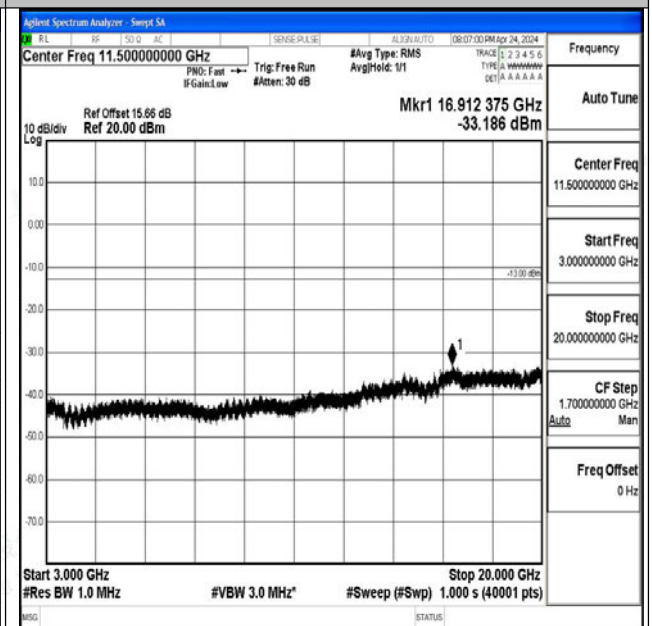
Band66_10MHz_16QAM_132622_1RB#0_3000~20000_3000~20000 3000~20000
