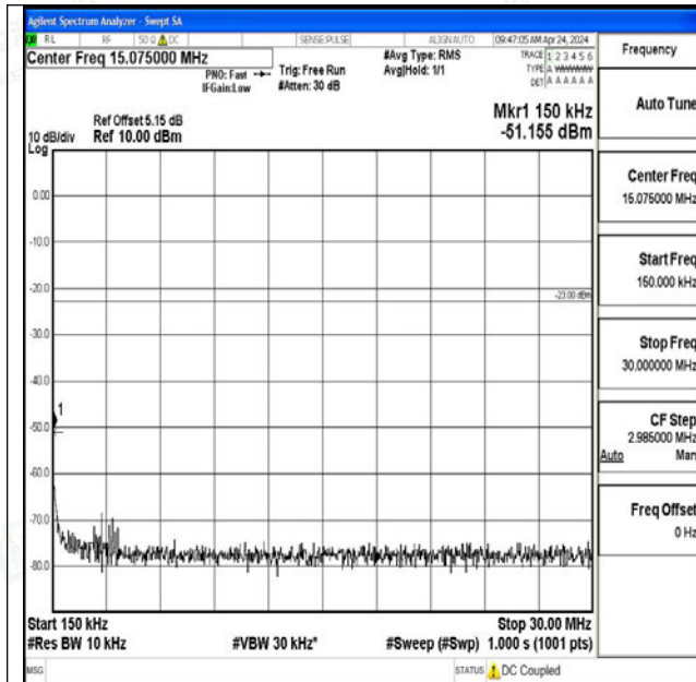
Band12_10MHz_16QAM_23130_1RB#0_0.15~30_0.15~30
