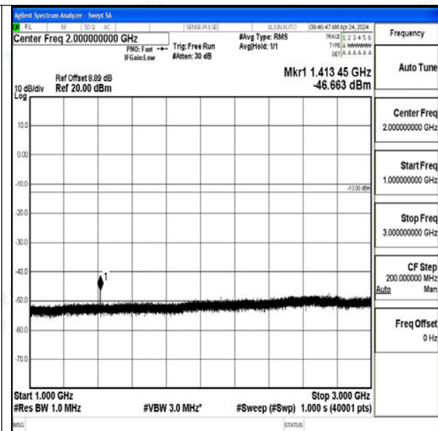
Band12_10MHz_QPSK_23130_1RB#0_1000~3000_1000~3000
