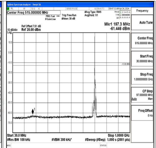
Band12_10MHz_16QAM_23130_1RB#0_30~1000_30~1000
