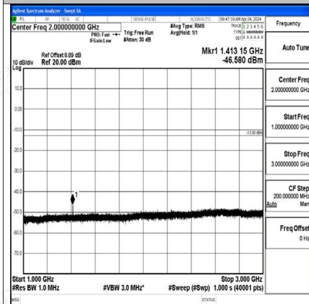
Band12_10MHz_16QAM_23130_1RB#0_1000~3000_1000~3000
