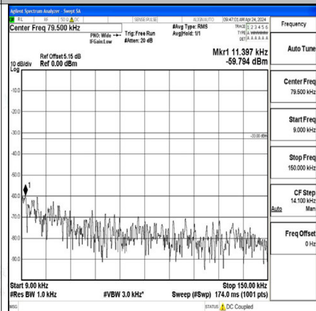
Band12_10MHz_16QAM_23130_1RB#0_0.009~0.15_0.009~0.15
