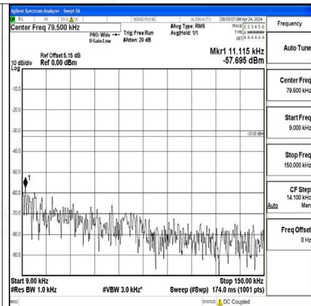
Band12_3MHz_16QAM_23095_1RB#0_0.009~0.15_0.0 09~0.15
