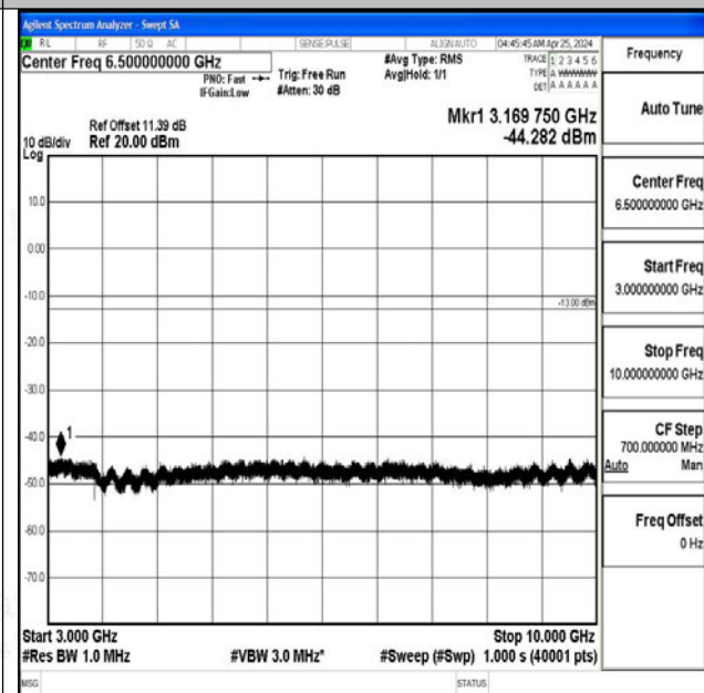
Band12_1.4MHz_16QAM_23095_1RB#0_3000~10000_ 3000~10000
