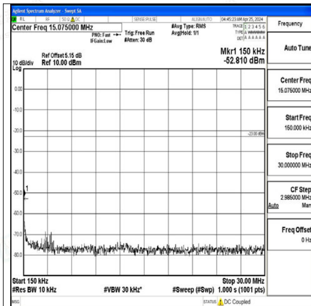
Band12_1.4MHz_16QAM_23095_1RB#0_0.15~30_0.15 ~30
