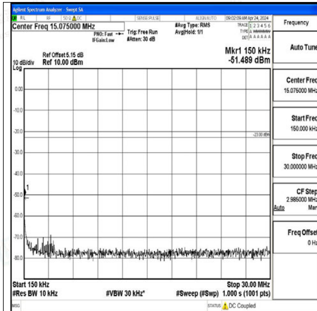
Band12_3MHz_16QAM_23025_1RB#0_0.15~30_0.15~3
