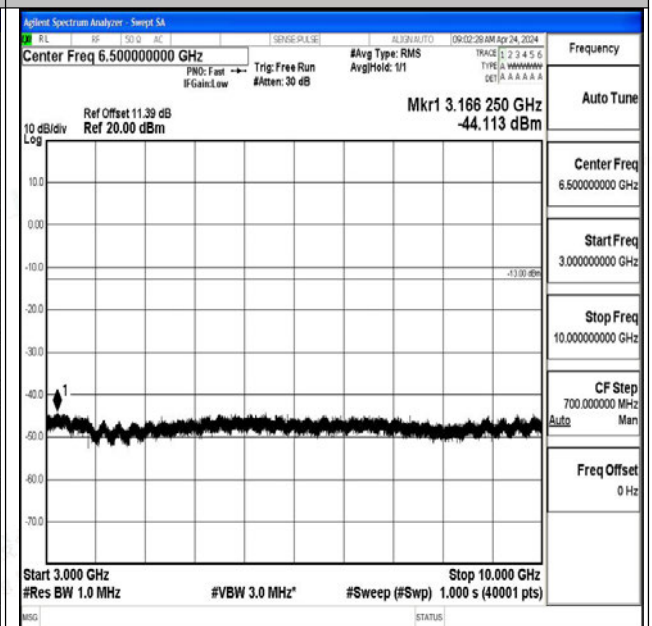
Band12_3MHz_16QAM_23025_1RB#0_3000~10000_30
