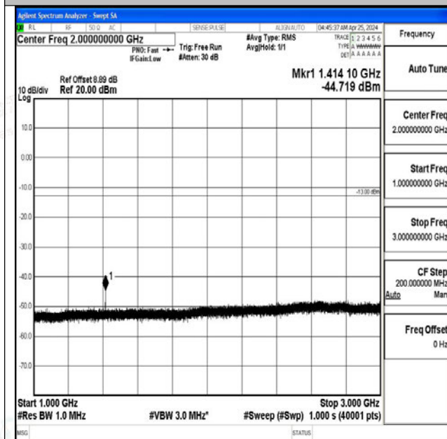
Band12_1.4MHz_16QAM_23095_1RB#0_1000~3000_1 000~3000
