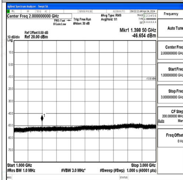
Band12_3MHz_16QAM_23025_1RB#0_1000~3000_100
