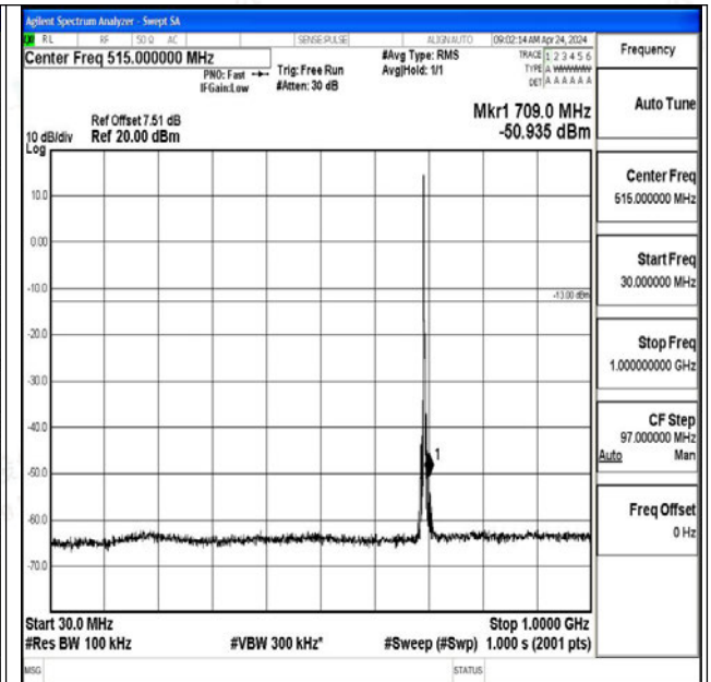
Band12_3MHz_16QAM_23025_1RB#0_30~1000_30~10
