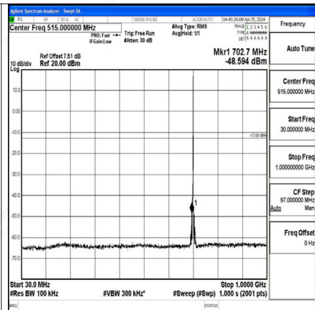
Band12_1.4MHz_16QAM_23095_1RB#0_30~1000_30~ 1000
