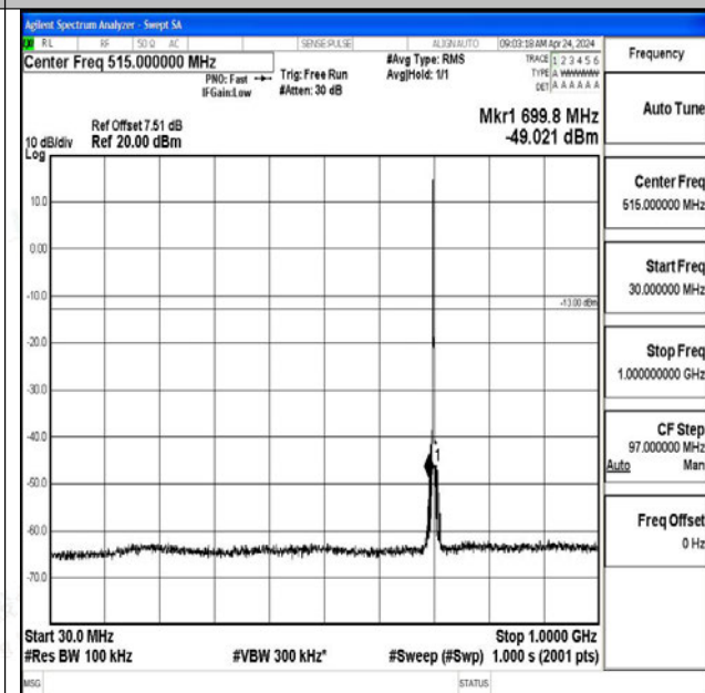
Band12_3MHz_16QAM_23095_1RB#0_30~1000_30~10 00
