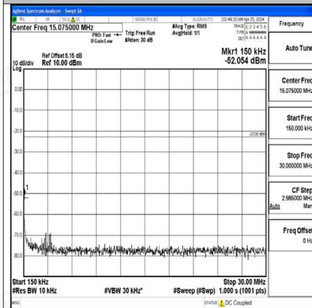
Band5_10MHz_16QAM_20525_1RB#0_0.15~30_0.15~3 0
