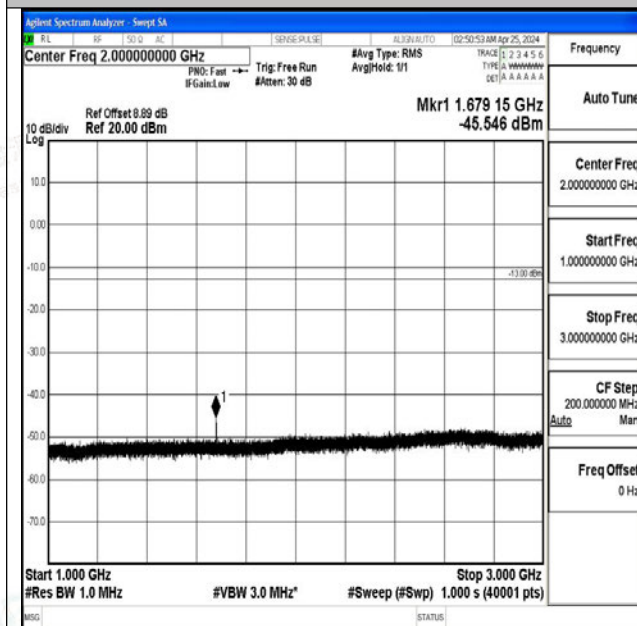
Band5_10MHz_16QAM_20600_1RB#0_1000~3000_100
