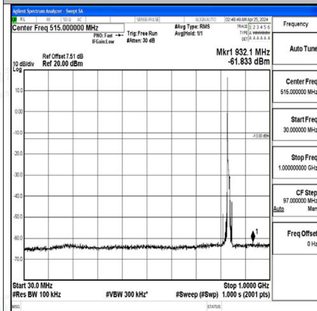
Band5_10MHz_QPSK_20525_1RB#0_30~1000_30~100 0
