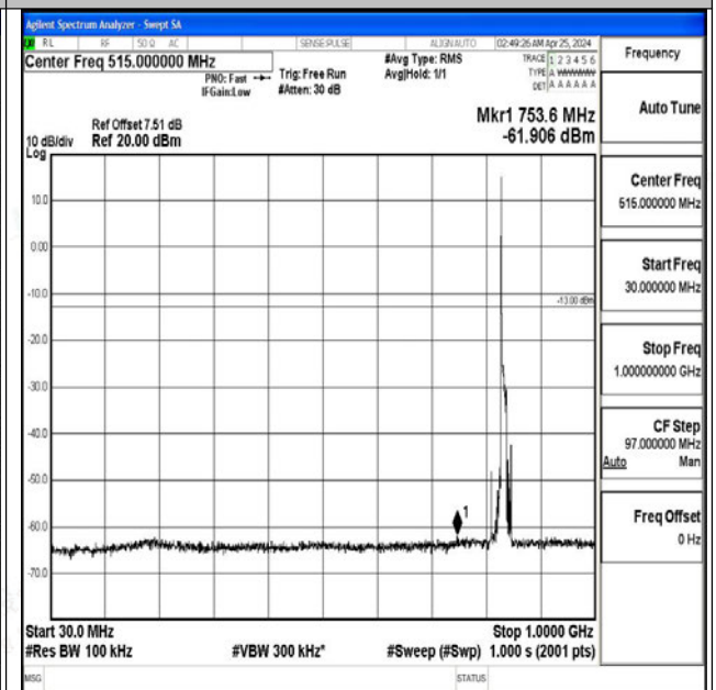
Band5_10MHz_16QAM_20525_1RB#0_30~1000_30~10 00
