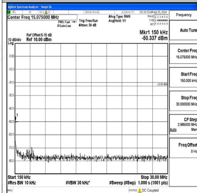
Band5_1.4MHz_16QAM_20643_1RB#0_0.15~30_0.15~30 30
