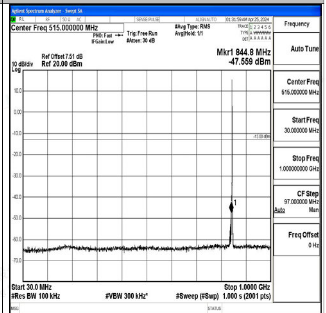
Band5_1.4MHz_16QAM_20643_1RB#0_30~1000_30~1000 000
