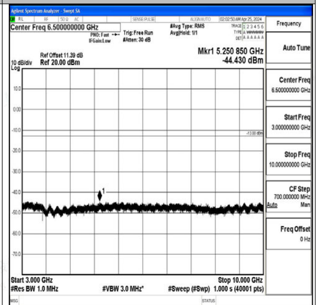
Band5_3MHz_16QAM_20635_1RB#0_3000~10000_3000~10000
