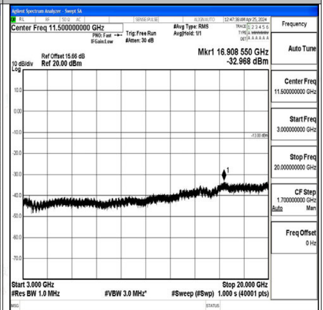
Band4_15MHz_QPSK_20175_1RB#0_3000~20000_3000 0~20000
