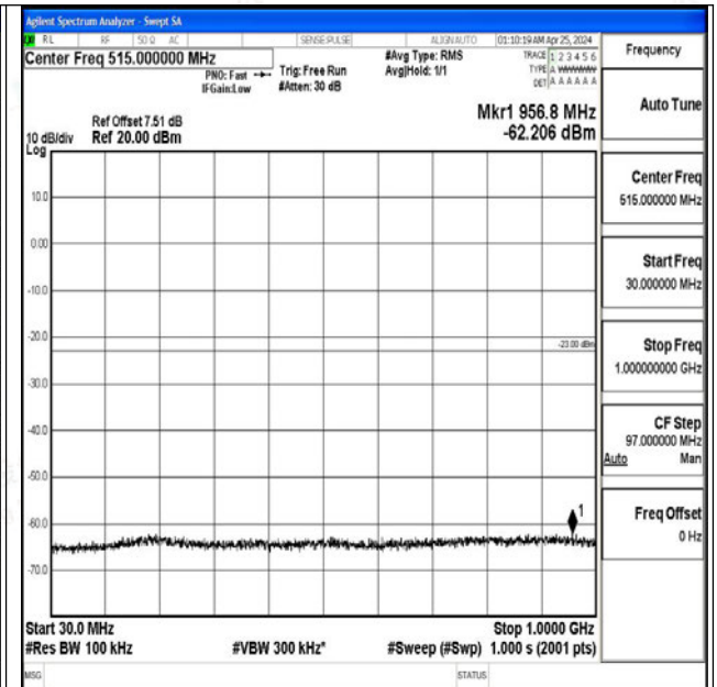
Band4_20MHz_QPSK_20300_1RB#0_30~1000_30~1000 0
