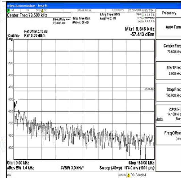
Band4_20MHz_16QAM_20300_1RB#0_0.009~0.15_0.0 09~0.15
