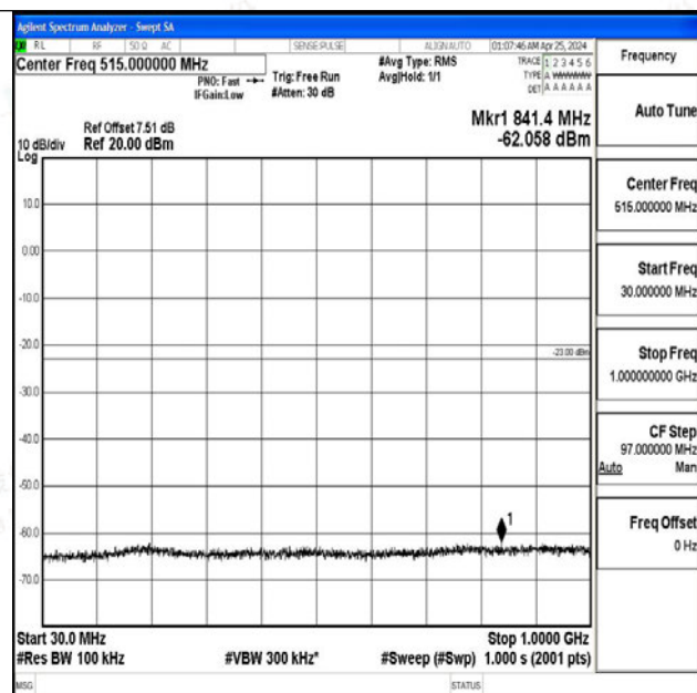
Band4_20MHz_QPSK_20050_1RB#0_30~1000_30~1000 0
