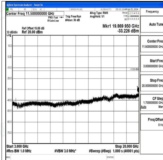
Band4_20MHz_16QAM_20300_1RB#0_3000~20000_3000~20000
