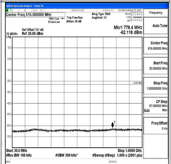
Band4_20MHz_QPSK_20175_1RB#0_30~1000_30~1000 0
