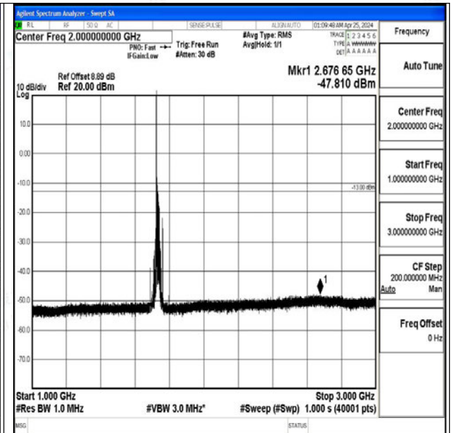
Band4_20MHz_16QAM_20175_1RB#0_1000~3000_1000~3000
