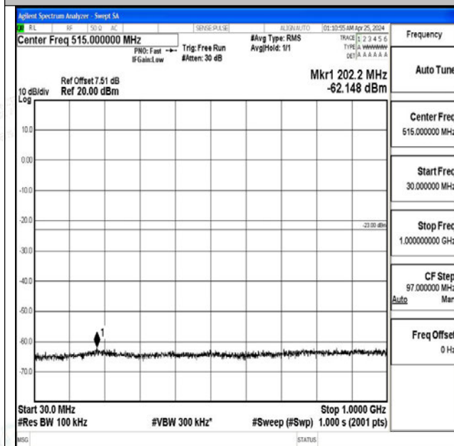
Band4_20MHz_16QAM_20300_1RB#0_30~1000_30~10 00
