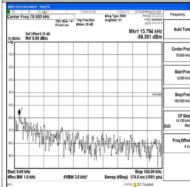
Band4_20MHz_16QAM_20175_1RB#0_0.009~0.15_0.0 09~0.15
