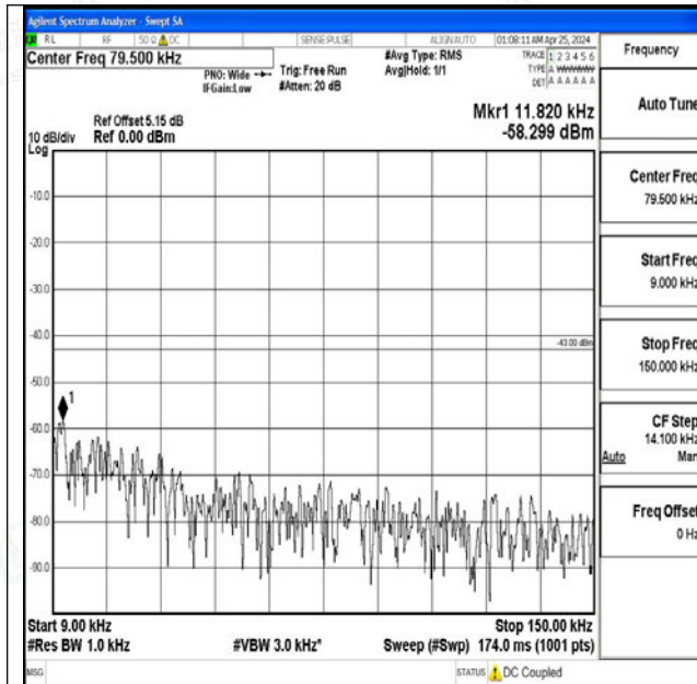
Band4_20MHz_16QAM_20050_1RB#0_0.009~0.15_0.0 09~0.15
