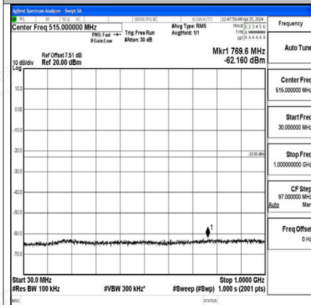
Band4_15MHz_16QAM_20175_1RB#0_30~1000_30~10 00
