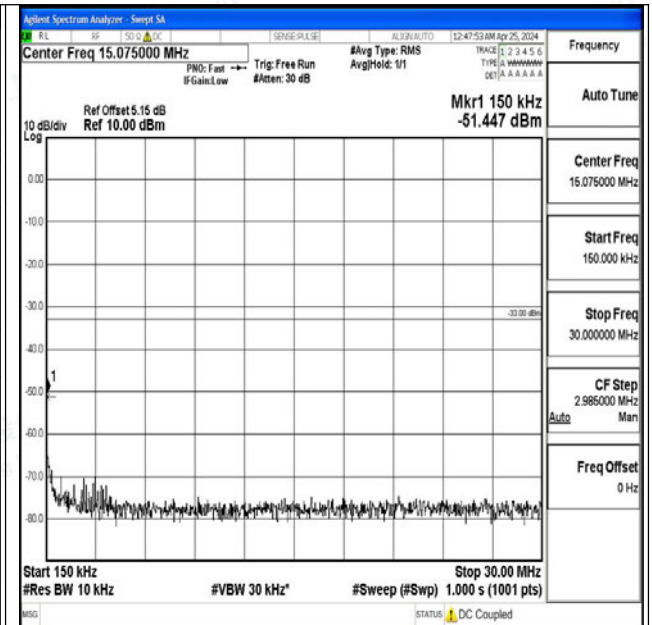
Band4_15MHz_16QAM_20175_1RB#0_0.15~30_0.15~3 0
