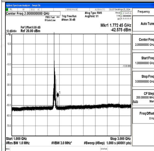
Band4_20MHz_QPSK_20050_1RB#0_1000~3000_1000 ~3000
