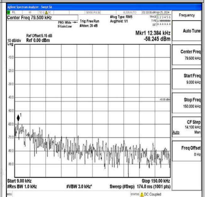
Band4_20MHz_QPSK_20300_1RB#0_0.009~0.15_0.009~0.15
