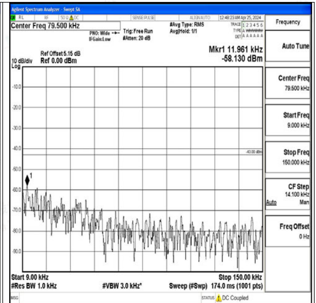
Band4_15MHz_QPSK_20325_1RB#0_0.009~0.15_0.009~0.15
