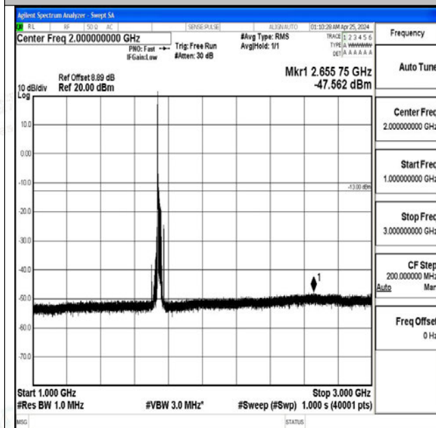
Band4_20MHz_QPSK_20300_1RB#0_1000~3000_1000 ~3000
