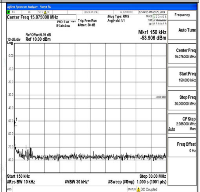
Band4_15MHz_16QAM_20325_1RB#0_0.15~30_0.15~3 0
