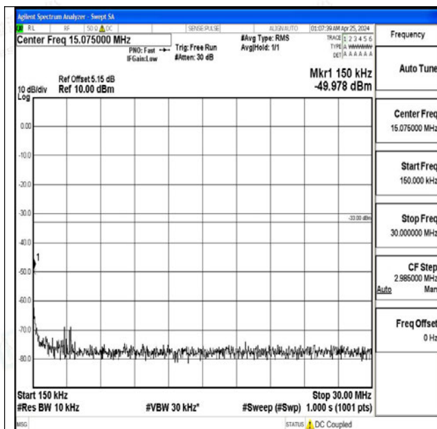
Band4_20MHz_QPSK_20050_1RB#0_0.15~30_0.15~30
