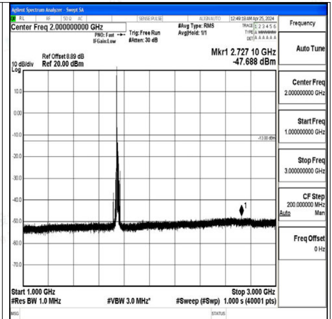
Band4_15MHz_16QAM_20325_1RB#0_1000~3000_1000~3000
