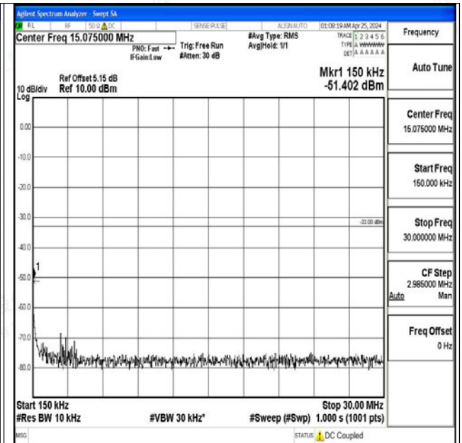
Band4_20MHz_16QAM_20050_1RB#0_0.15~30_0.15~3 0
