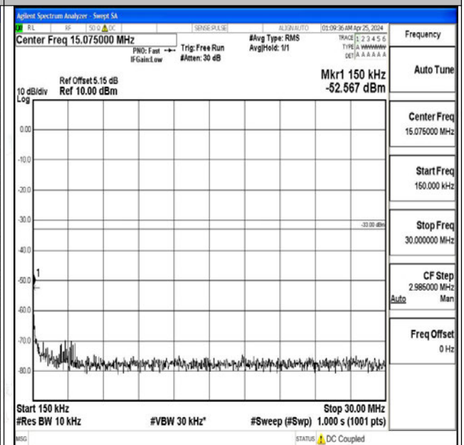
Band4_20MHz_16QAM_20175_1RB#0_0.15~30_0.15~3 0
