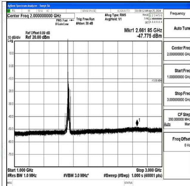
Band4_20MHz_QPSK_20175_1RB#0_1000~3000_1000 ~3000
