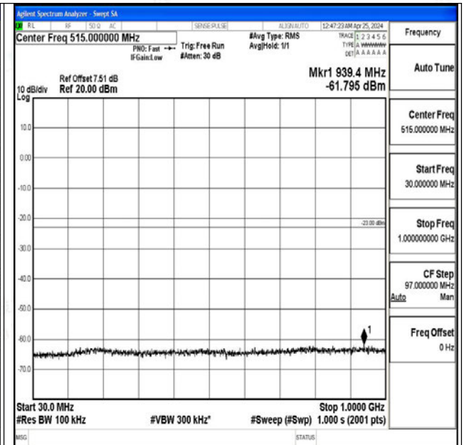
Band4_15MHz_QPSK_20175_1RB#0_30~1000_30~1000 0
