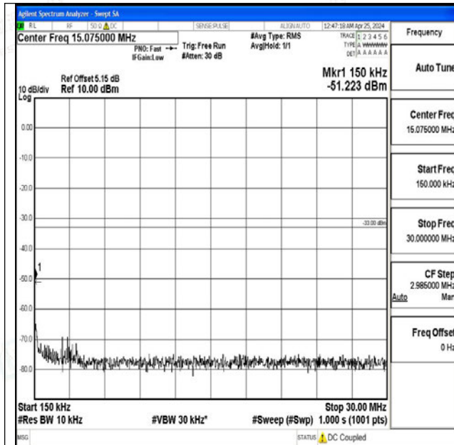
Band4_15MHz_QPSK_20175_1RB#0_0.15~30_0.15~30
