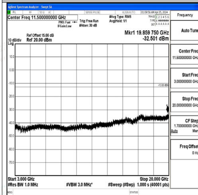
Band4_20MHz_16QAM_20175_1RB#0_3000~20000_3000~20000
