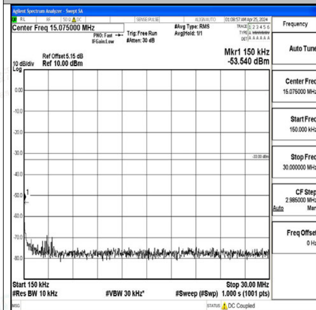
Band4_20MHz_16QAM_20050_1RB#0_3000~20000_3000~20000
