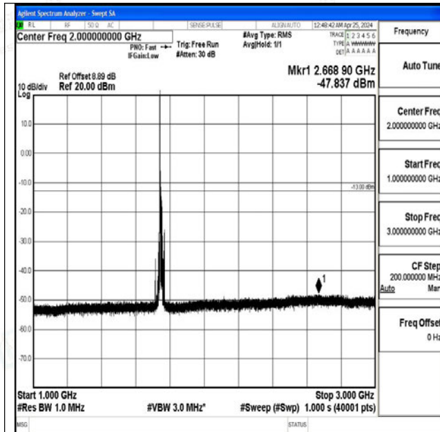
Band4_15MHz_QPSK_20325_1RB#0_1000~3000_1000 ~3000
