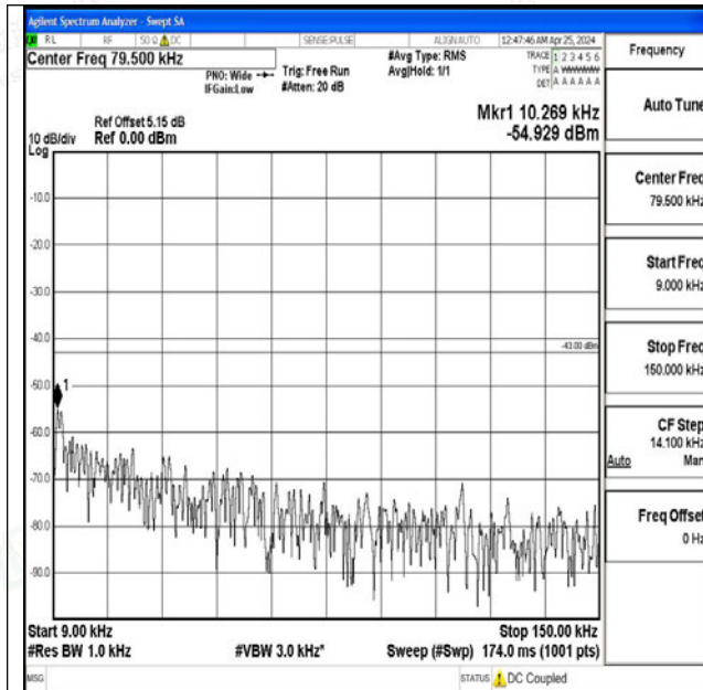
Band4_15MHz_16QAM_20175_1RB#0_0.009~0.15_0.0 09~0.15
