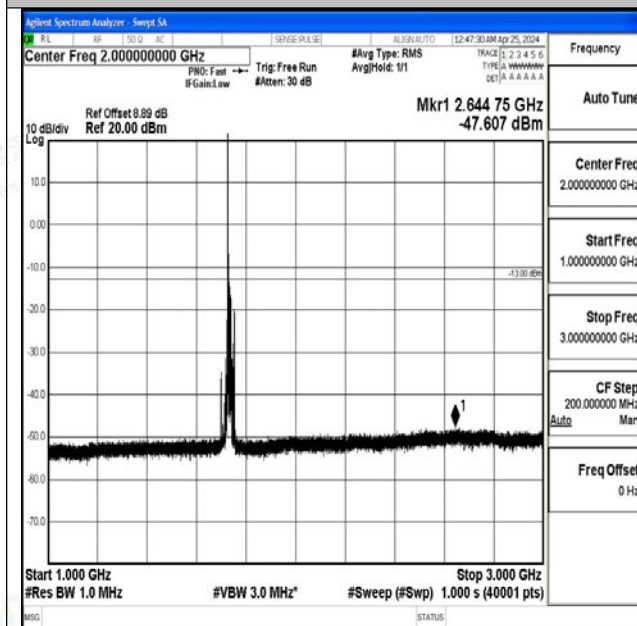
Band4_15MHz_QPSK_20175_1RB#0_1000~3000_1000 ~3000
