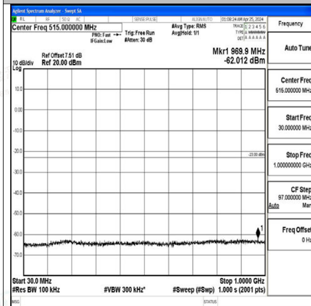
Band4_20MHz_16QAM_20050_1RB#0_30~1000_30~10 00
