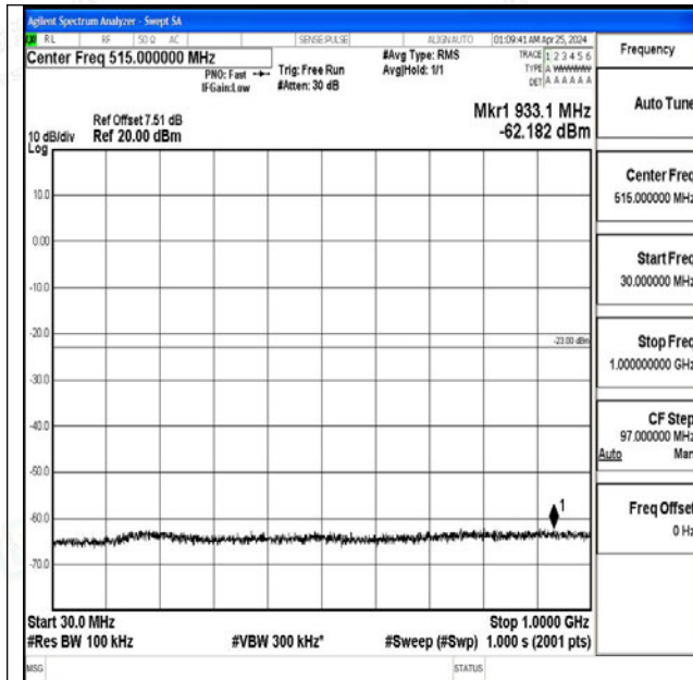
Band4_20MHz_16QAM_20175_1RB#0_30~1000_30~1000
