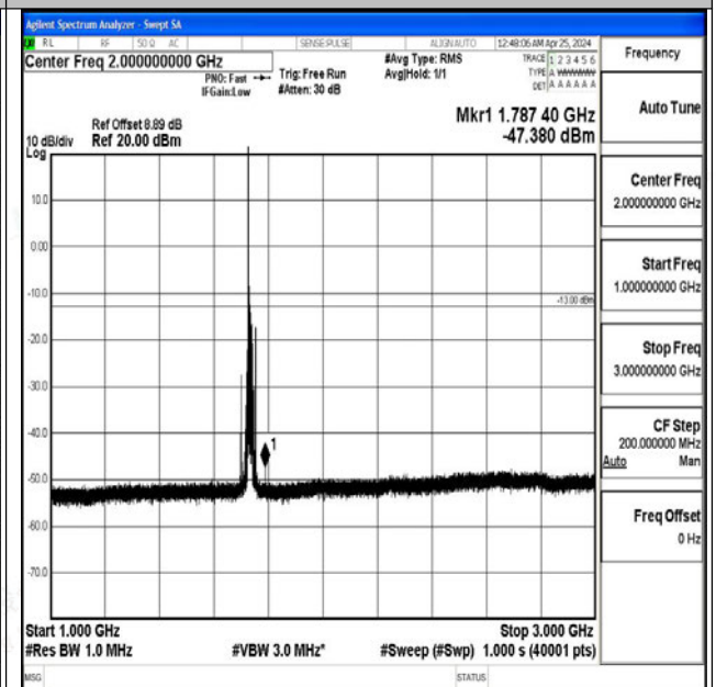
Band4_15MHz_16QAM_20175_1RB#0_1000~3000_100 0~3000
