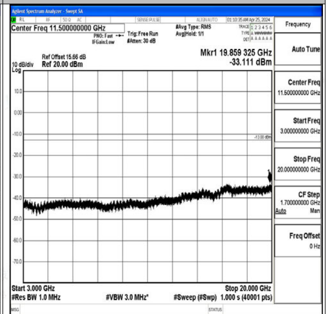
Band4_20MHz_QPSK_20300_1RB#0_3000~20000_3000 0~20000
