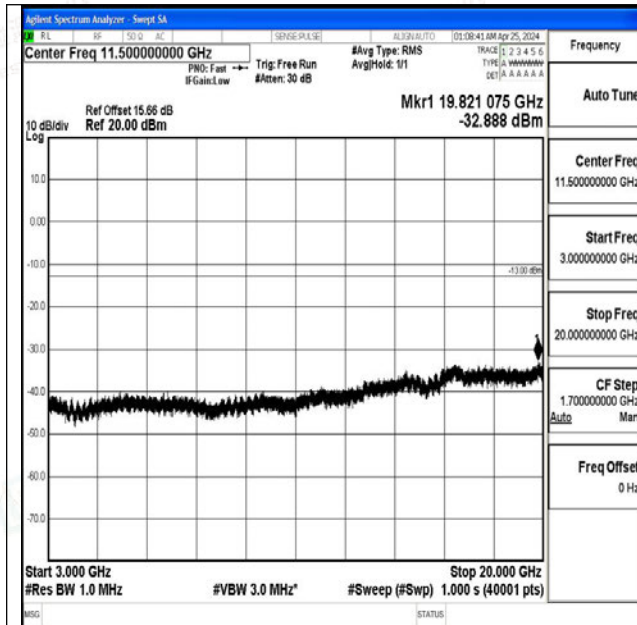
Band4_20MHz_16QAM_20050_1RB#0_3000~20000_3000~20000
