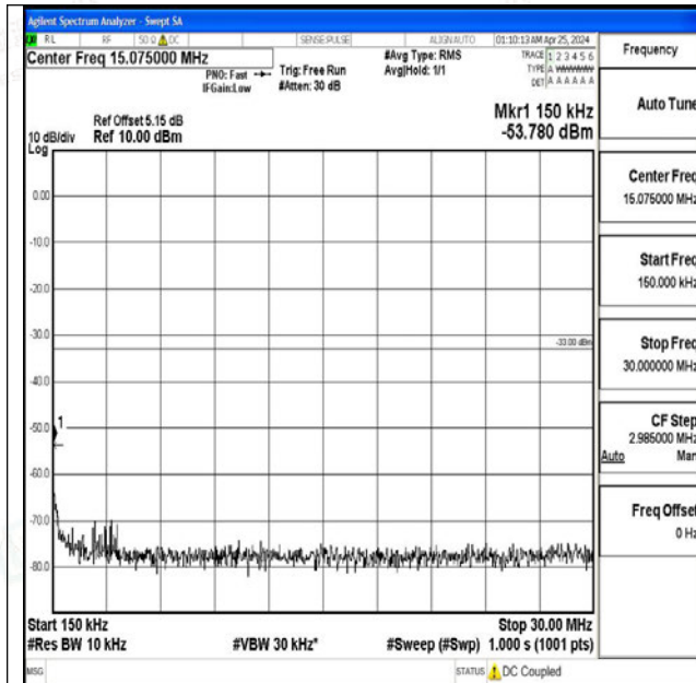
Band4_20MHz_QPSK_20300_1RB#0_0.15~30_0.15~30
