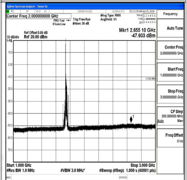
Band4_20MHz_16QAM_20300_1RB#0_1000~3000_100 0~3000
