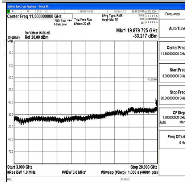
Band4_15MHz_16QAM_20325_1RB#0_3000~20000_3000~20000
