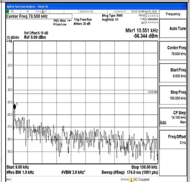
Band4_20MHz_QPSK_20050_1RB#0_0.009~0.15_0.009~0.15
