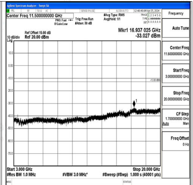
Band4_15MHz_QPSK_20325_1RB#0_3000~20000_300 0~20000
