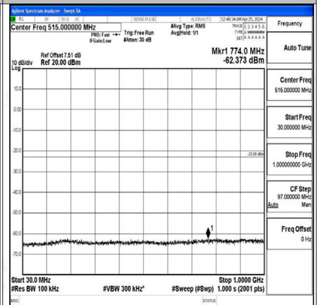
Band4_15MHz_QPSK_20325_1RB#0_30~1000_30~1000
