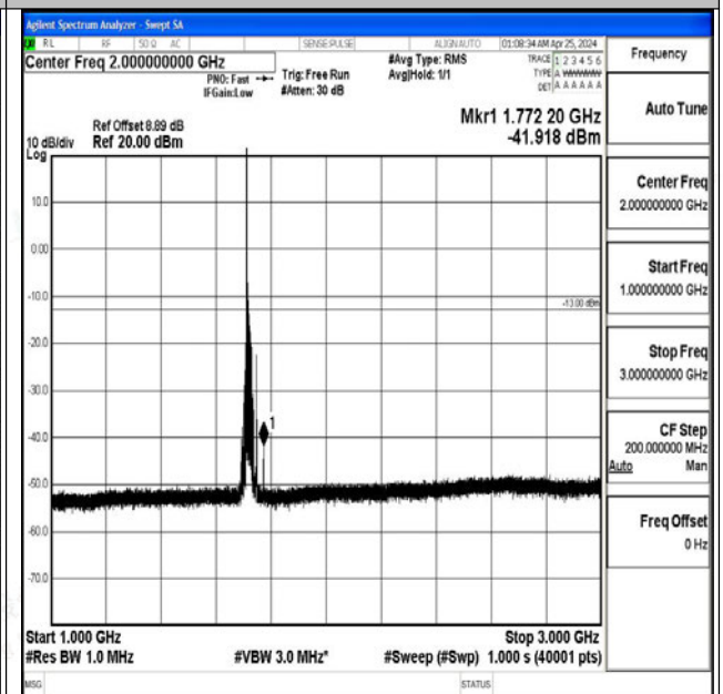
Band4_20MHz_16QAM_20050_1RB#0_1000~3000_100 0~3000
