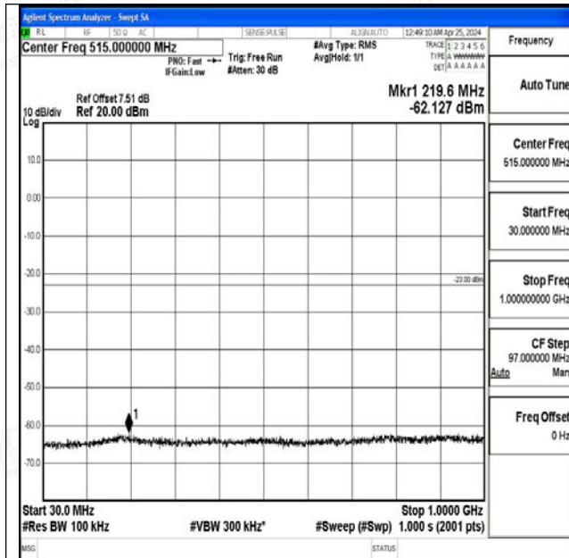
Band4_15MHz_16QAM_20325_1RB#0_30~1000_30~1000
