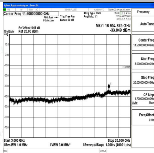
Band4_20MHz_QPSK_20050_1RB#0_3000~20000_3000 0~20000
