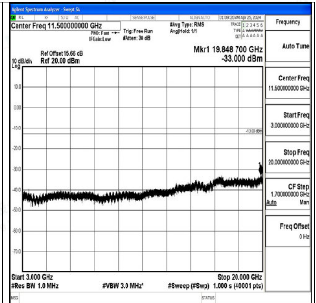
Band4_20MHz_QPSK_20175_1RB#0_3000~20000_300 0~20000
