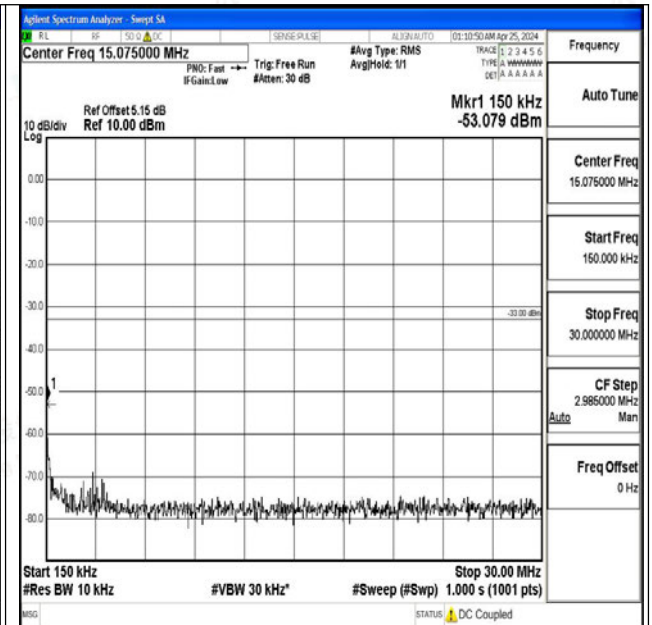
Band4_20MHz_16QAM_20300_1RB#0_0.15~30_0.15~3 0
