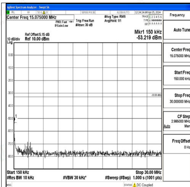
Band4_10MHz_QPSK_20000_1RB#0_0.15~30_0.15~30
