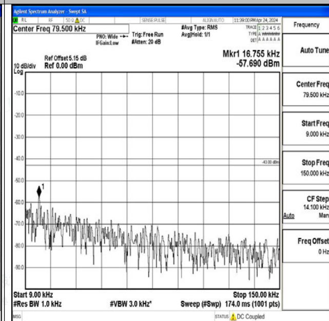
Band4_3MHz_16QAM_19965_1RB#0_0.009~0.15_0.009~0.15
