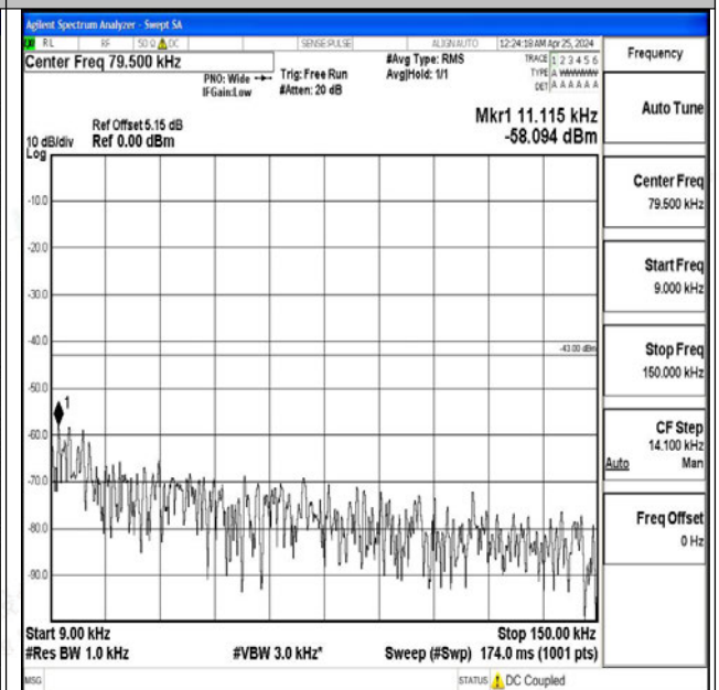
Band4_10MHz_QPSK_20000_1RB#0_0.009~0.15_0.009~0.15 ~0.15
