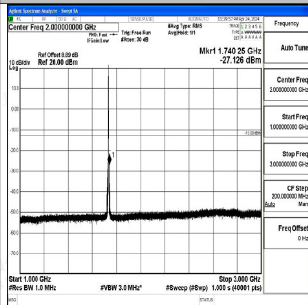
Band4_3MHz_QPSK_20175_1RB#0_1000~3000_1000~3000
