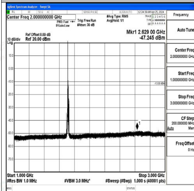
Band4_10MHz_QPSK_20000_1RB#0_1000~3000_1000 ~3000
