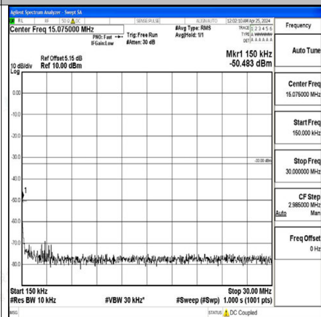
Band4_5MHz_16QAM_19975_1RB#0_0.15~30_0.15~30
