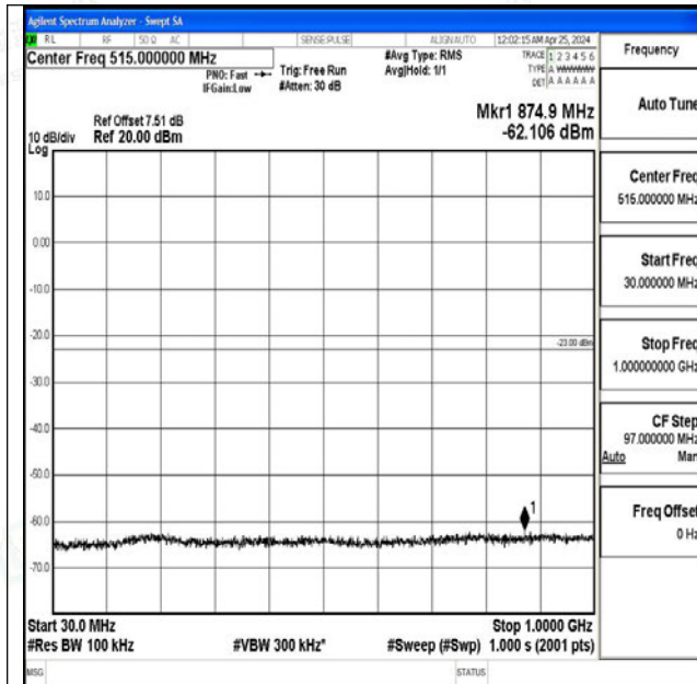
Band4_5MHz_16QAM_19975_1RB#0_30~1000_30~100
