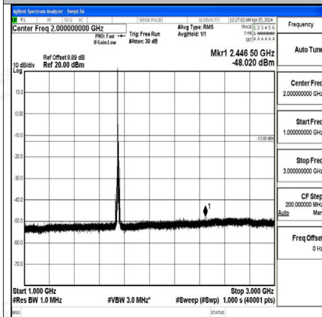
Band4_10MHz_QPSK_20350_1RB#0_1000~3000_1000 ~3000
