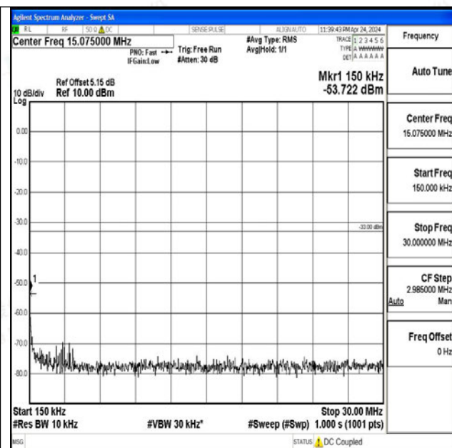
Band4_3MHz_QPSK_20175_1RB#0_0.15~30_0.15~30
