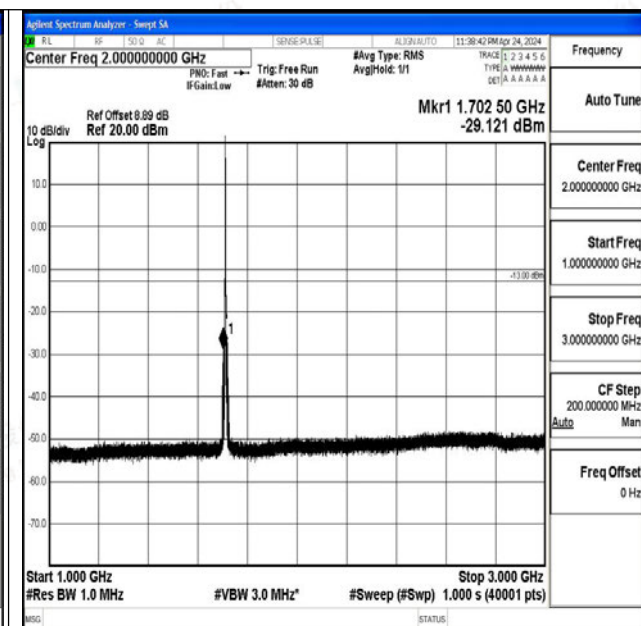
Band4_3MHz_QPSK_19965_1RB#0_1000~3000_1000~3000
