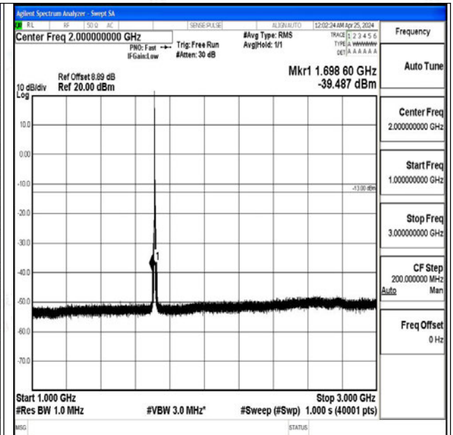
Band4_5MHz_16QAM_19975_1RB#0_1000~3000_1000
