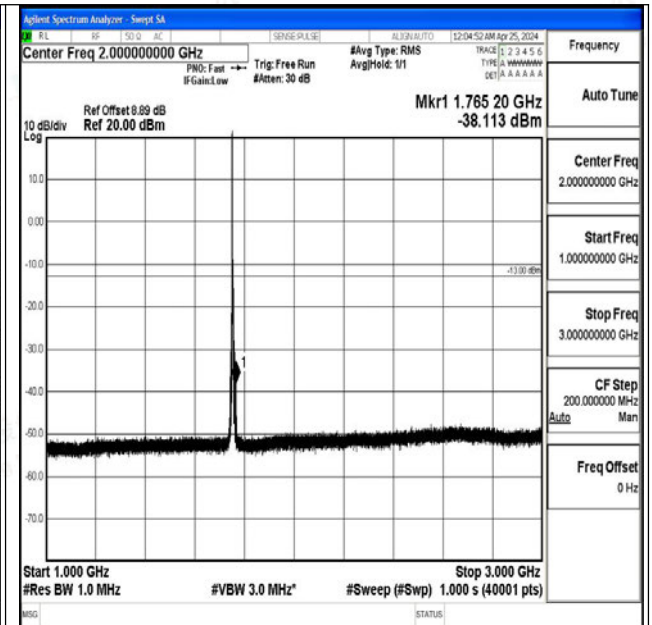
Band4_5MHz_16QAM_20375_1RB#0_1000~3000_1000~3000 ~3000
