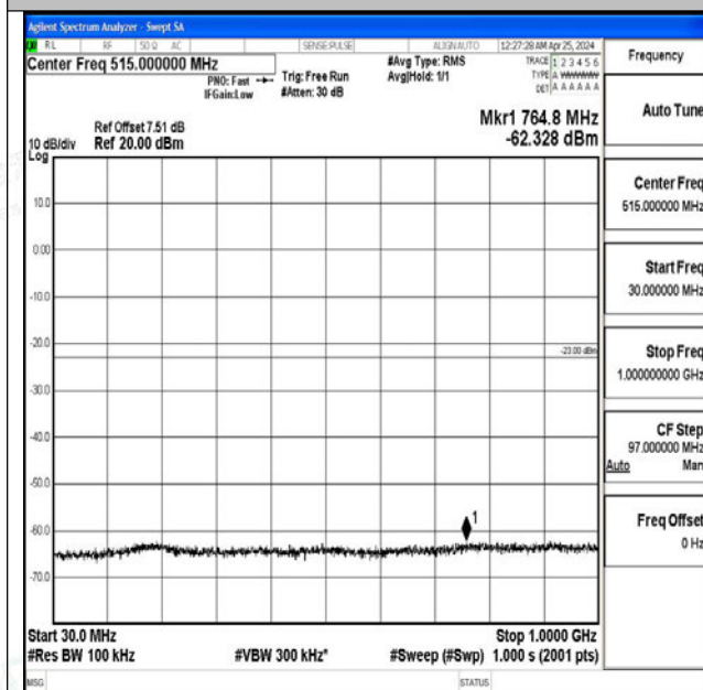
Band4_10MHz_16QAM_20350_1RB#0_30~1000_30~10 00
