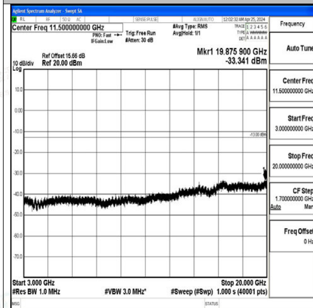
Band4_5MHz_16QAM_19975_1RB#0_3000~20000_300
