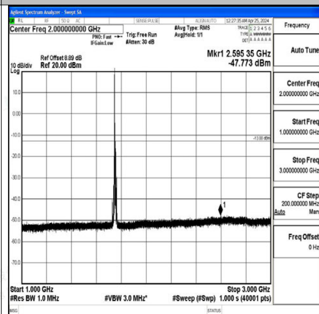
Band4_10MHz_16QAM_20350_1RB#0_1000~3000_100 0~3000
