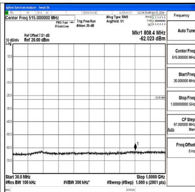
Band4_10MHz_QPSK_20000_1RB#0_30~1000_30~1000 0
