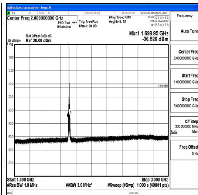
Band4_5MHz_QPSK_19975_1RB#0_1000~3000_1000~3000
