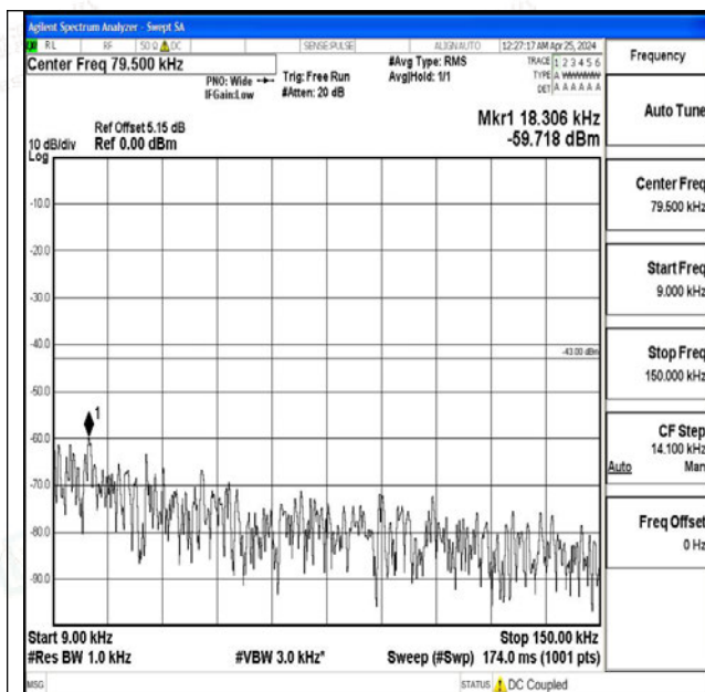
Band4_10MHz_16QAM_20350_1RB#0_0.009~0.15_0.0 09~0.15
