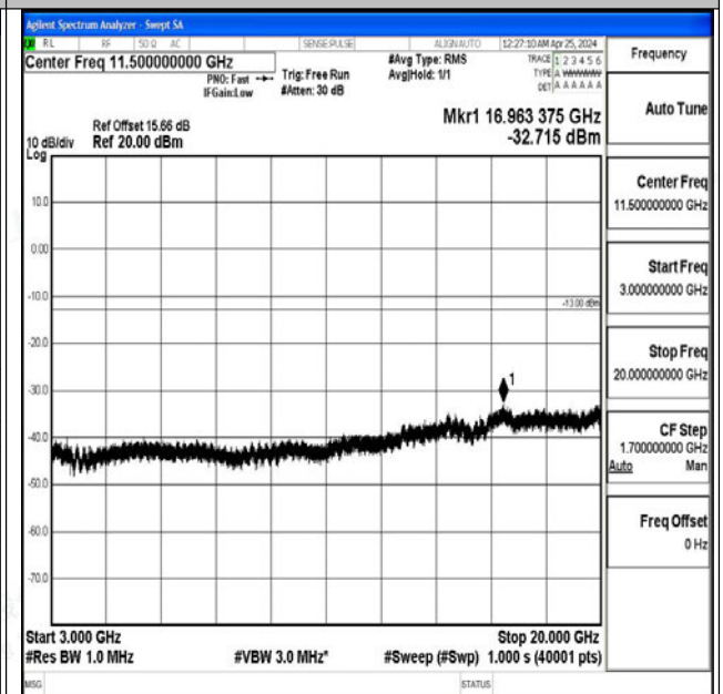
Band4_10MHz_QPSK_20350_1RB#0_3000~20000_3000 0~20000
