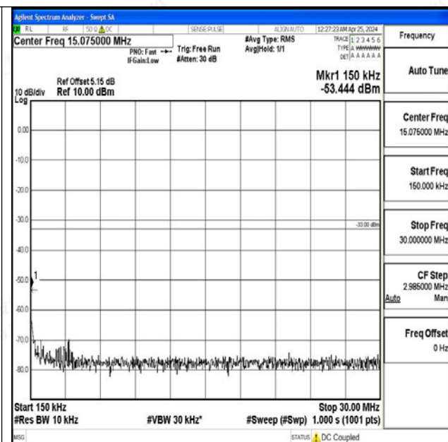
Band4_10MHz_16QAM_20350_1RB#0_0.15~30_0.15~3 0
