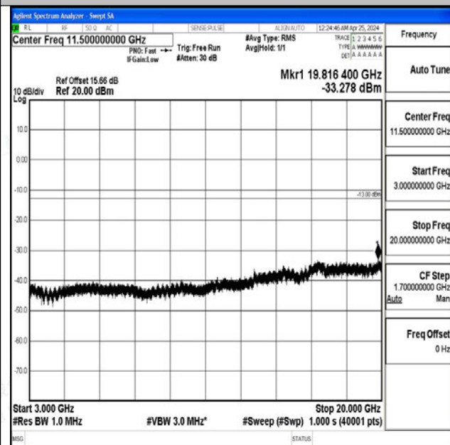
Band4_10MHz_QPSK_20000_1RB#0_3000~20000_3000 0~20000
