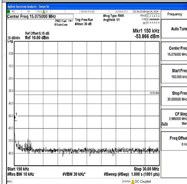
Band2_20MHz_16QAM_18900_1RB#0_0.15~30_0.15~3 0
