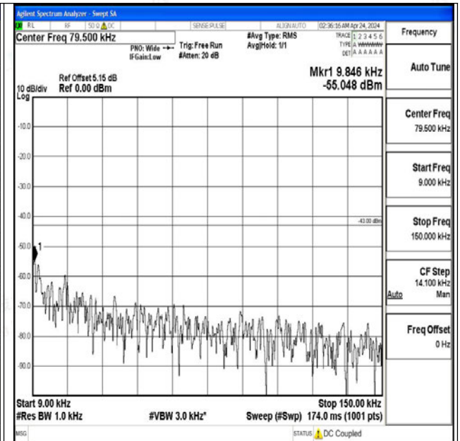
Band2_20MHz_16QAM_18900_1RB#0_0.009~0.15_0.0 09~0.15
