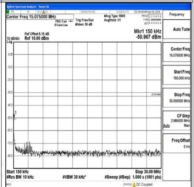
Band2_20MHz_QPSK_18700_1RB#0_0.15~30_0.15~30
