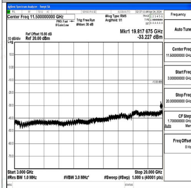
Band2_20MHz_QPSK_19100_1RB#0_3000~20000_300 0~20000
