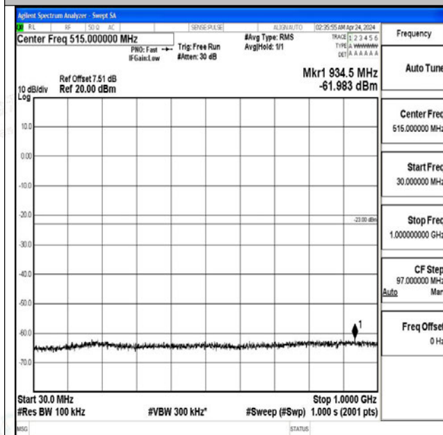
Band2_20MHz_QPSK_18900_1RB#0_30~1000_30~1000
