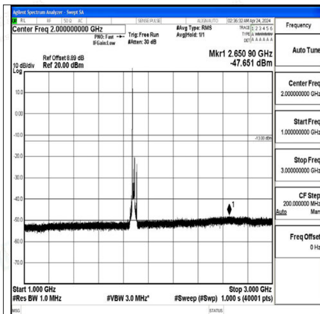
Band2_20MHz_16QAM_18900_1RB#0_1000~3000_100 0~3000
