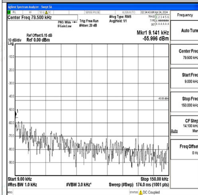
Band2_20MHz_QPSK_18700_1RB#0_0.009~0.15_0.009 ~0.15
