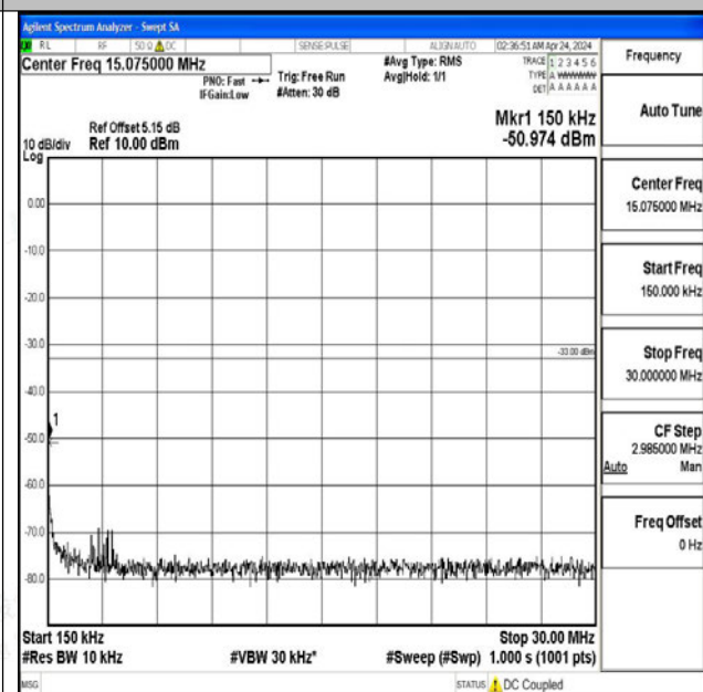
Band2_20MHz_QPSK_19100_1RB#0_0.15~30_0.15~30
