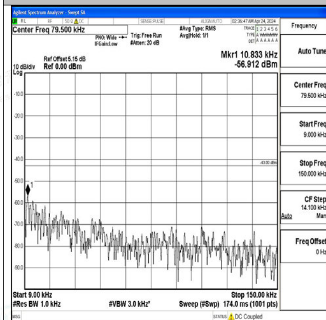
Band2_20MHz_QPSK_19100_1RB#0_0.009~0.15_0.009 ~0.15
