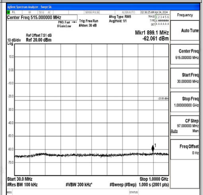
Band2_20MHz_16QAM_18900_1RB#0_30~1000_30~10 00
