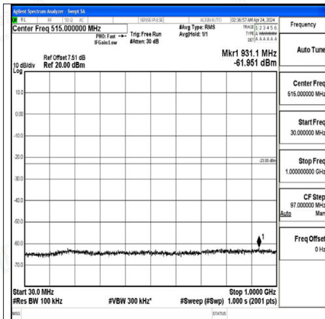
Band2_20MHz_QPSK_19100_1RB#0_30~1000_30~100 0
