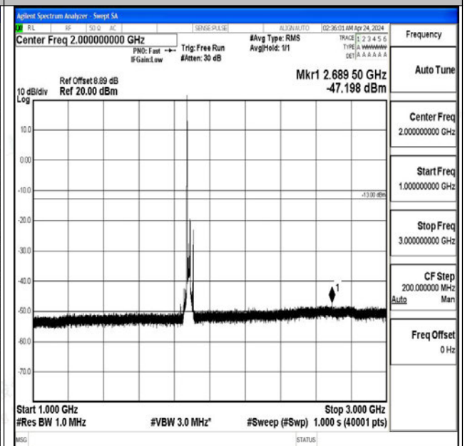
Band2_20MHz_QPSK_18900_1RB#0_1000~3000_1000~3000
