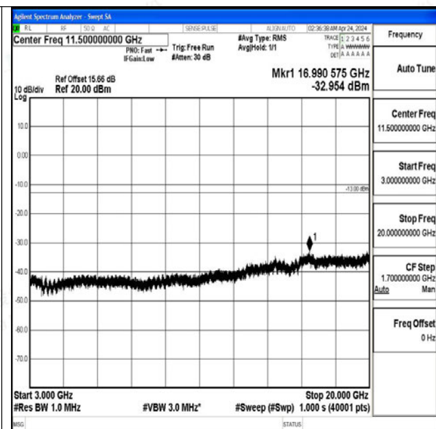
Band2_20MHz_16QAM_18900_1RB#0_3000~20000_30 00~20000
