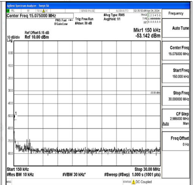
Band2_20MHz_QPSK_18900_1RB#0_0.15~30_0.15~30
