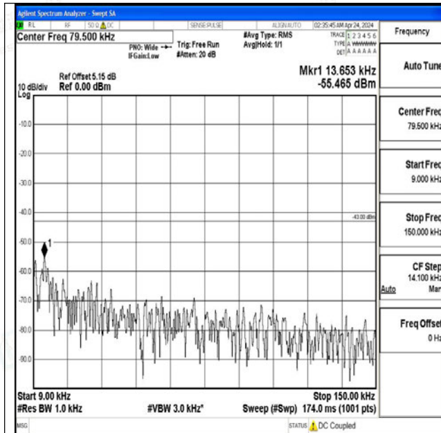
Band2_20MHz_QPSK_18900_1RB#0_0.009~0.15_0.009~0.15
