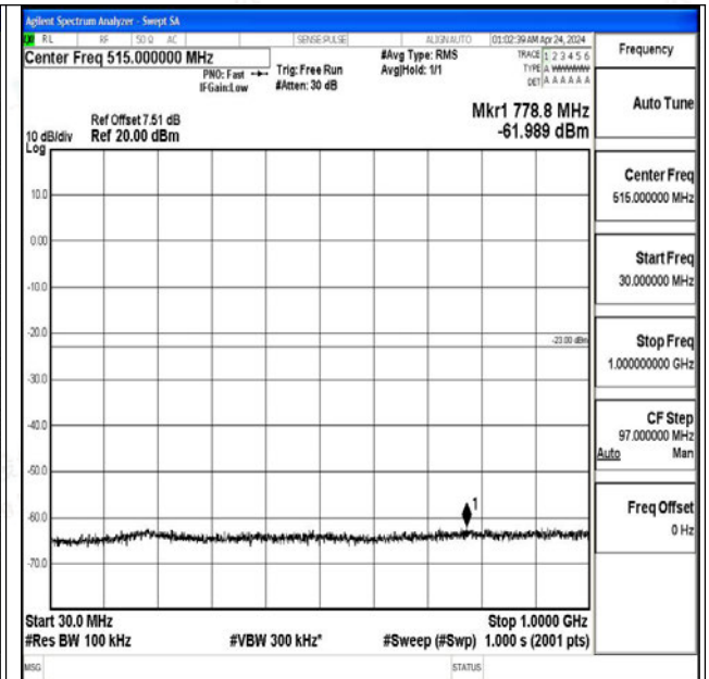
Band2_1.4MHz_16QAM_18900_1RB#0_30~1000_30~1000
