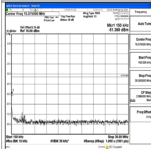
Band2_1.4MHz_16QAM_18607_1RB#0_0.15~30_0.15~ 30
