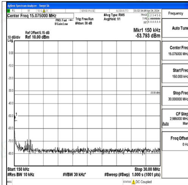
Band2_1.4MHz_16QAM_18900_1RB#0_0.15~30_0.15~30
