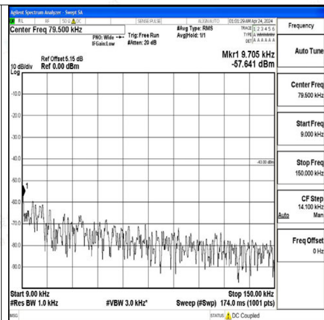
Band2_1.4MHz_16QAM_18607_1RB#0_0.009~0.15_0.0 09~0.15
