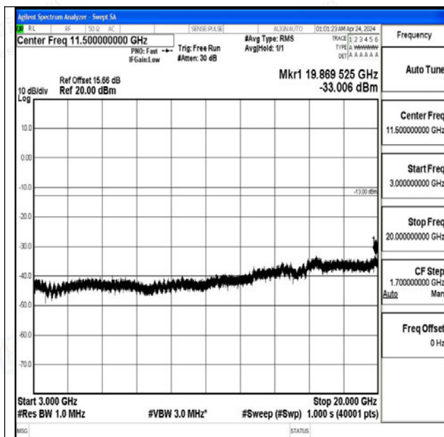
Band2_1.4MHz_QPSK_18607_1RB#0_3000~20000_300 0~20000
