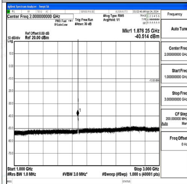
Band2_1.4MHz_16QAM_18900_1RB#0_1000~3000_1000~3000
