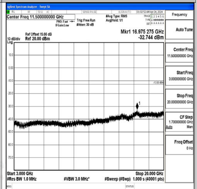
Band2_1.4MHz_16QAM_18900_1RB#0_3000~20000_3000~20000
