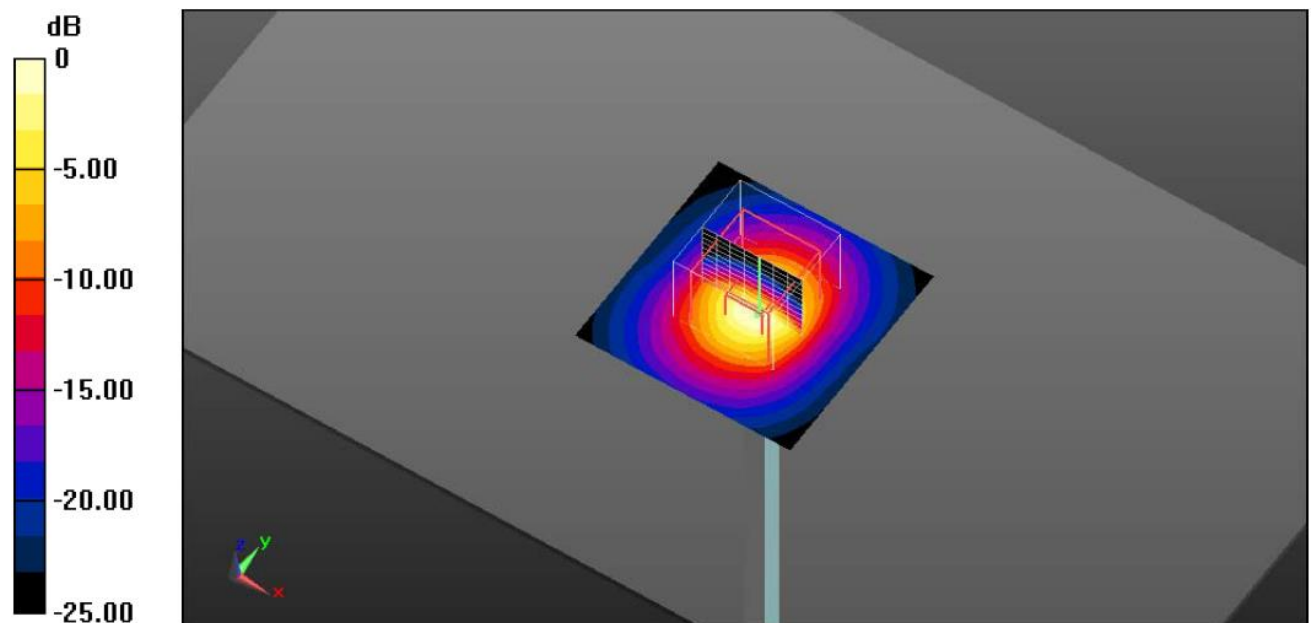
Plot 1: Body Test Position 2 (UHF RFID 900MHz Middle Channel)
