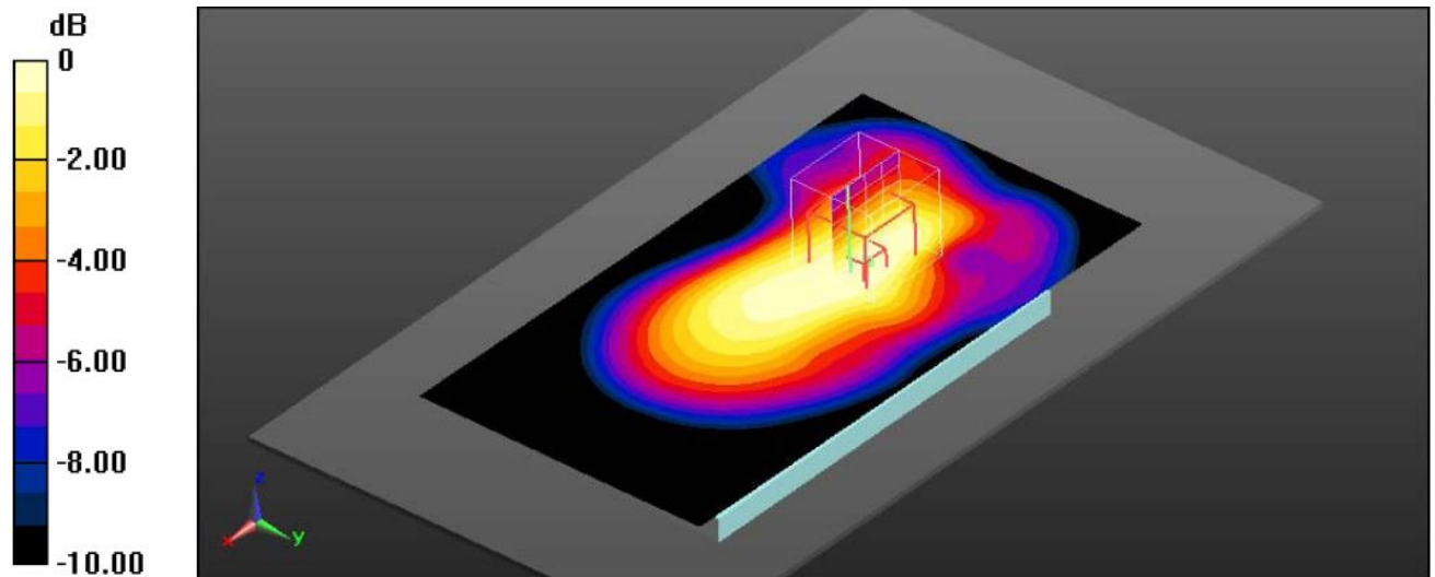
Plot 2: Body Test Position 5 (WiFi2450 Middle Channel-Channel 6-2437MHz (1Mbps))
