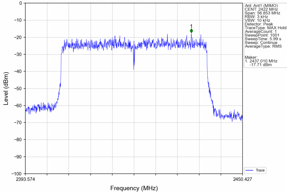
802.11ax(HEW40)_LCH_2422MHz_RU484_Left_MIMO_NTNV
