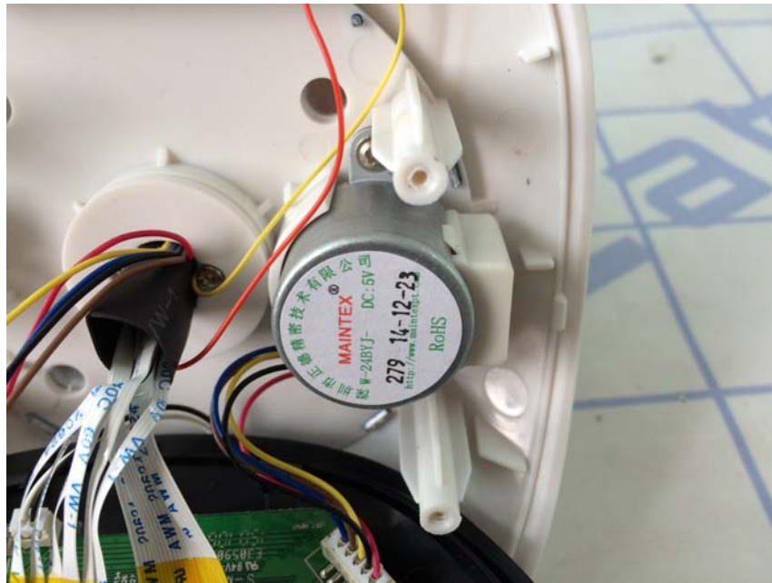
Motor view 1
