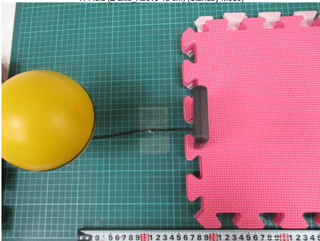
H-Field (Z-axis_Above 18 cm) (Standby Mode)
