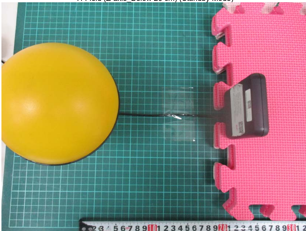
H-Field (Z-axis_Below 20 cm) (Standby Mode)
