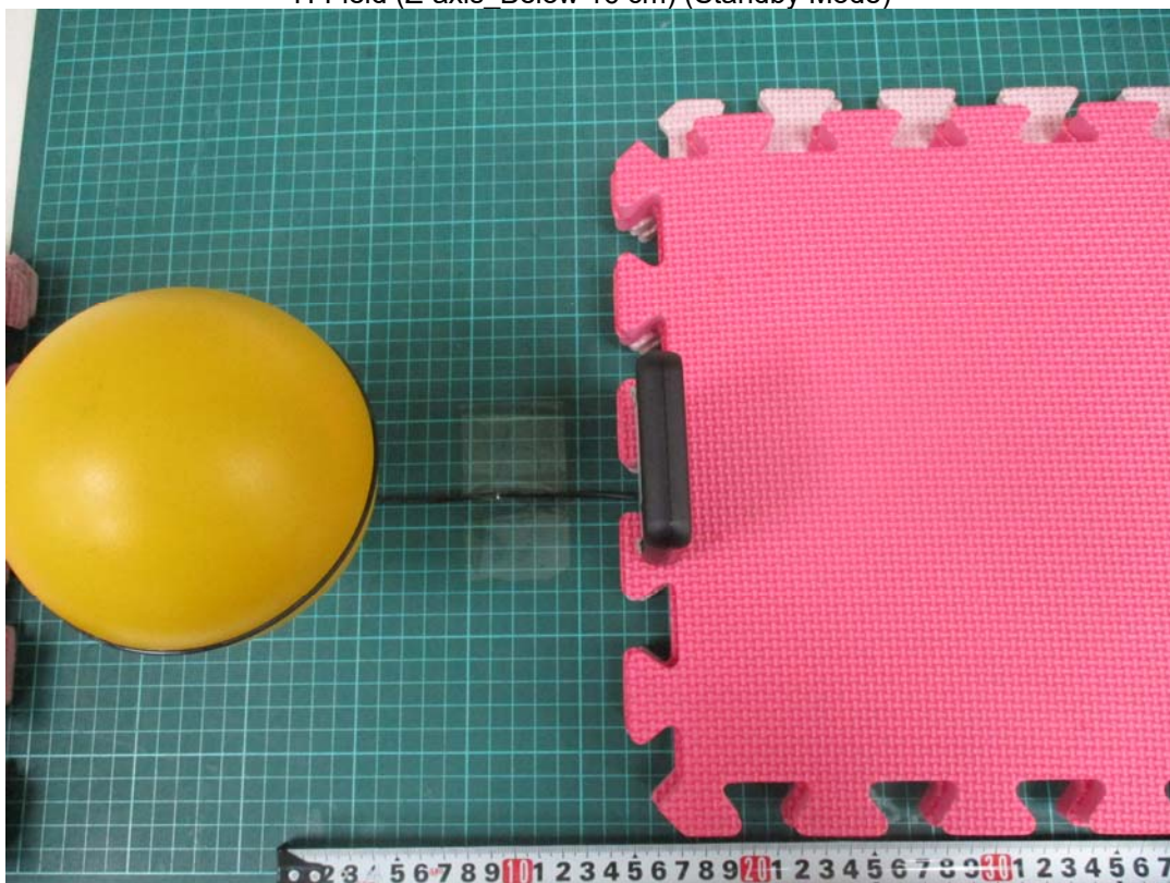
H-Field (Z-axis_Below 16 cm) (Standby Mode)
