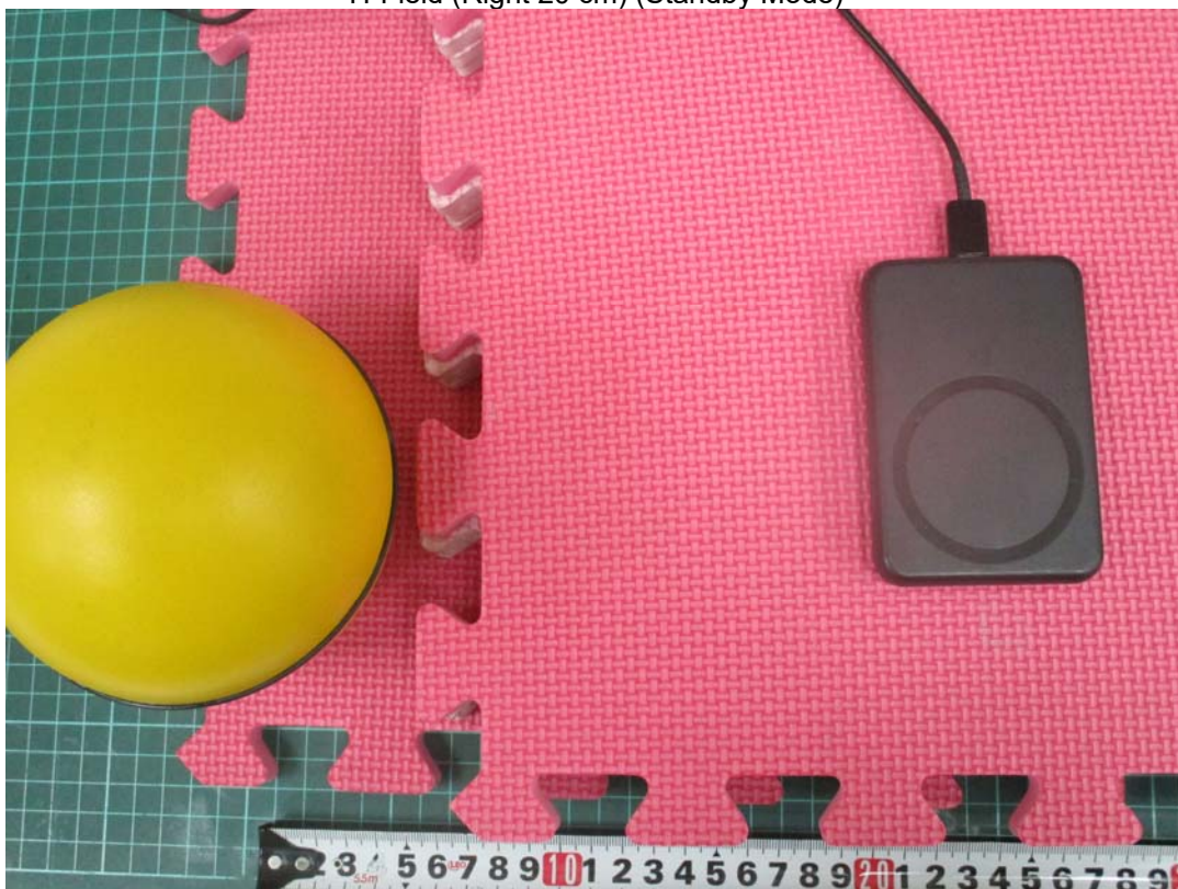
H-Field (Right 20 cm) (Standby Mode)
