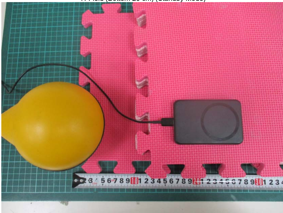
H-Field (Bottom 20 cm) (Standby Mode)
