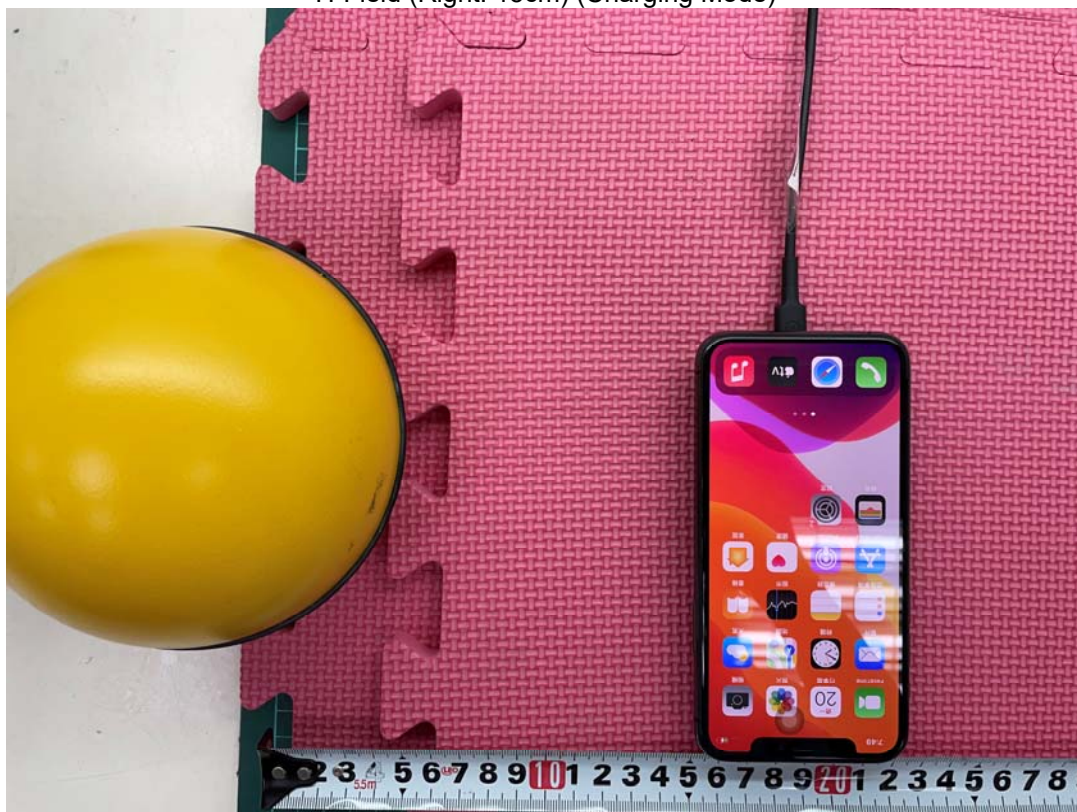
H-Field (Right: 15cm) (Charging Mode)
