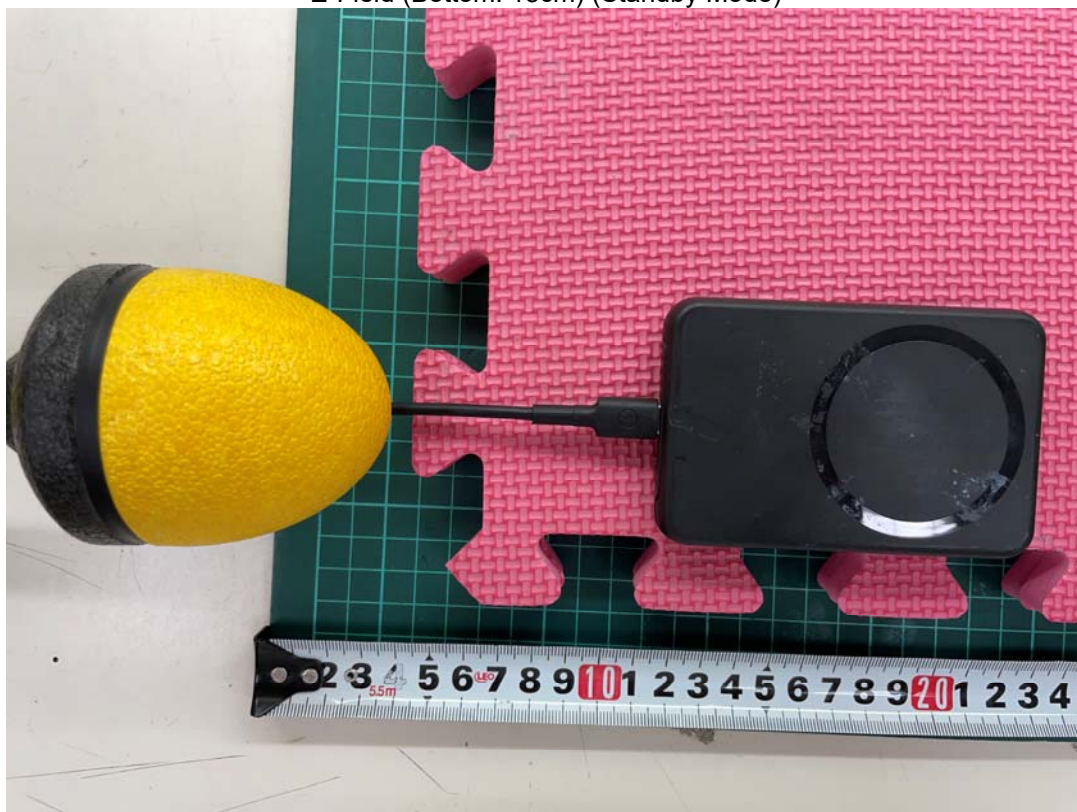
E-Field (Bottom: 15cm) (Standby Mode)
