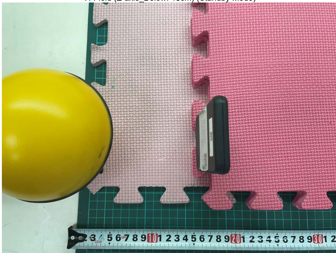
H-Field (Z-axis_Below: 15cm) (Standby Mode)
