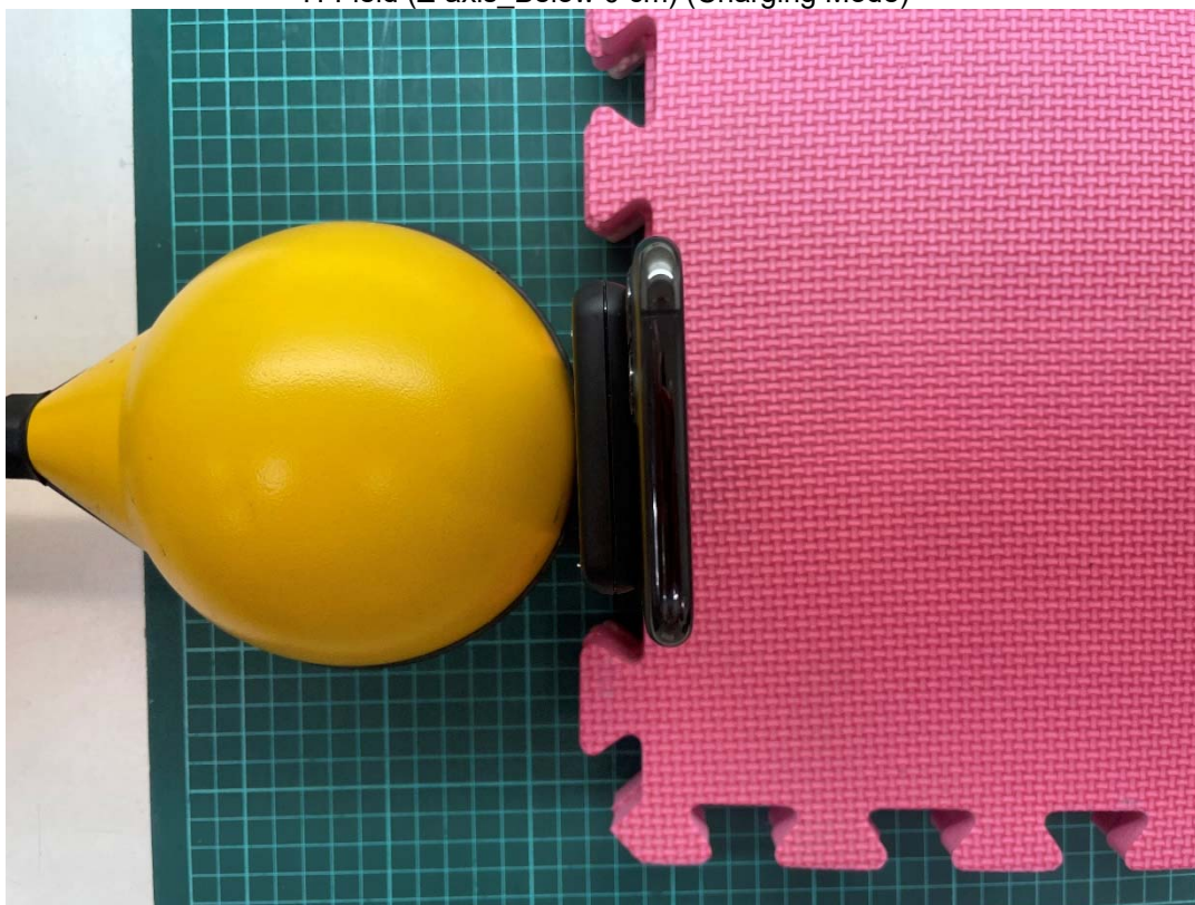
H-Field (Z-axis_Below 0 cm) (Charging Mode)
