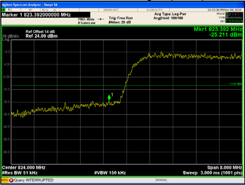
WCDMA band V band edge-left(HSUPA)
