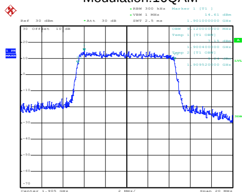
Modulation:16OAM
