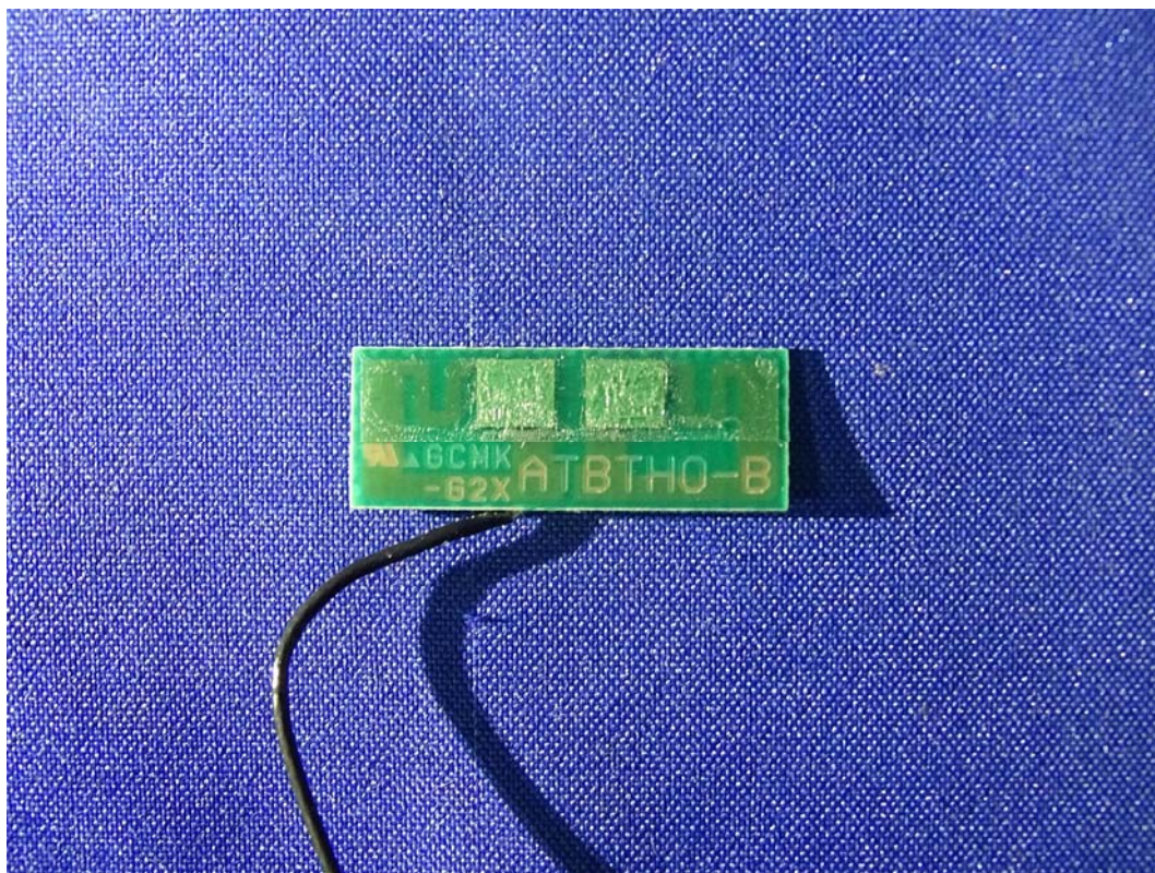
(34) EUT Photo-BT Antenna
