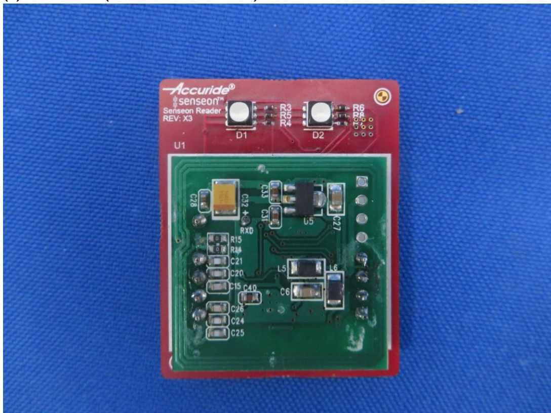
(2) EUT Photo (Senseon Plus Reader)
