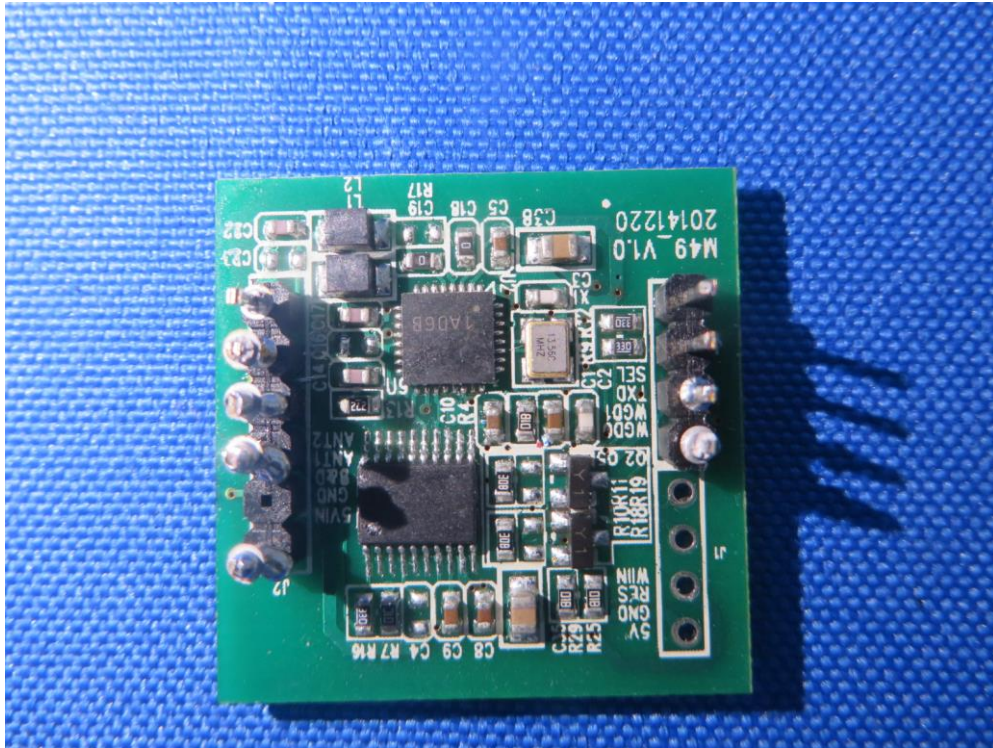
(5) EUT Photo (Senseon Plus Reader)
