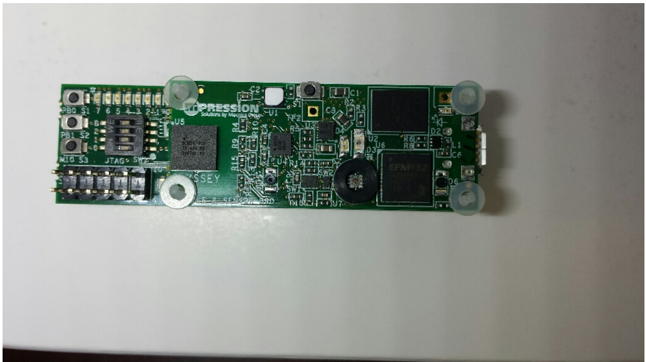
Alternate configuration without the max10 board but with battery board
