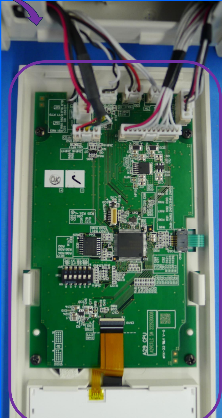
Open the CPU BOARD
