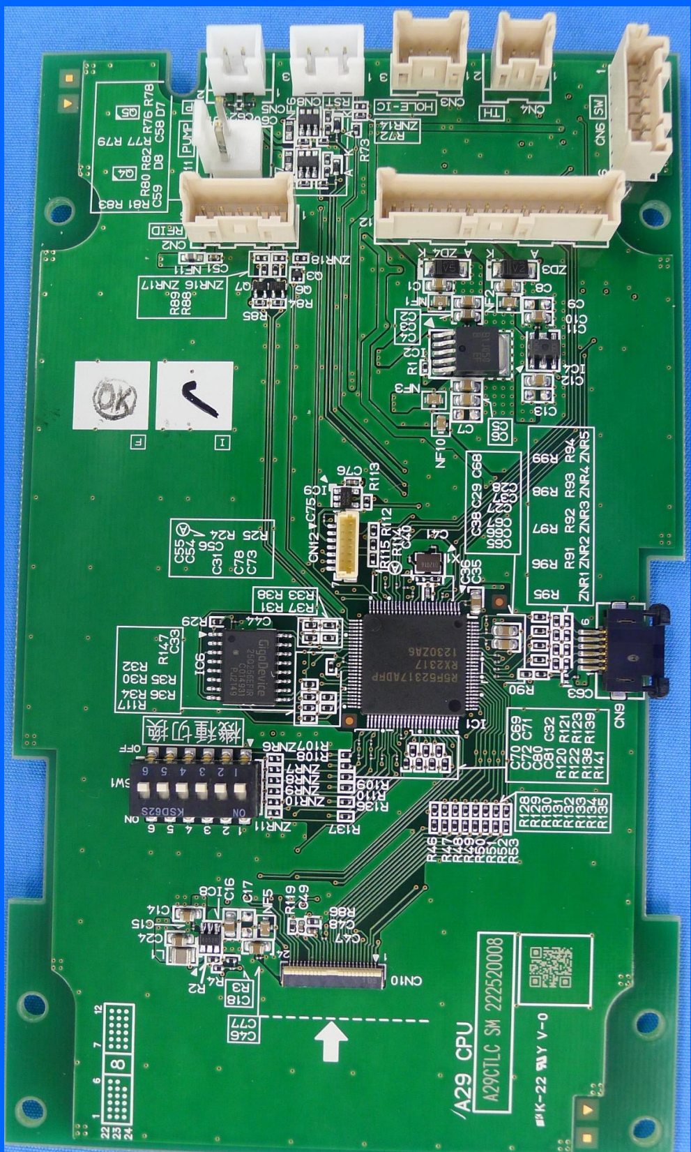
CPU BOARD Surface
