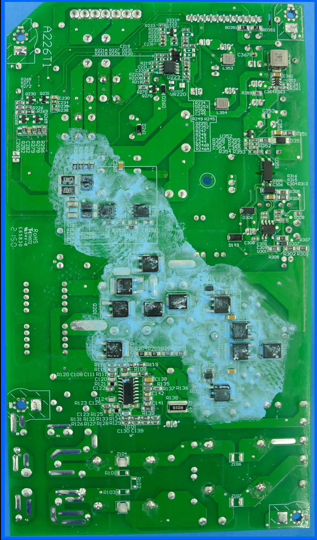
POWER SWITCHING BOARD back side
