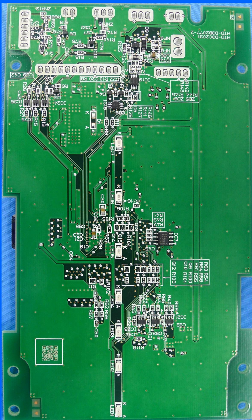
CPU BOARD back side
