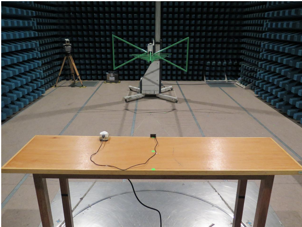
Charging mode (front view)
