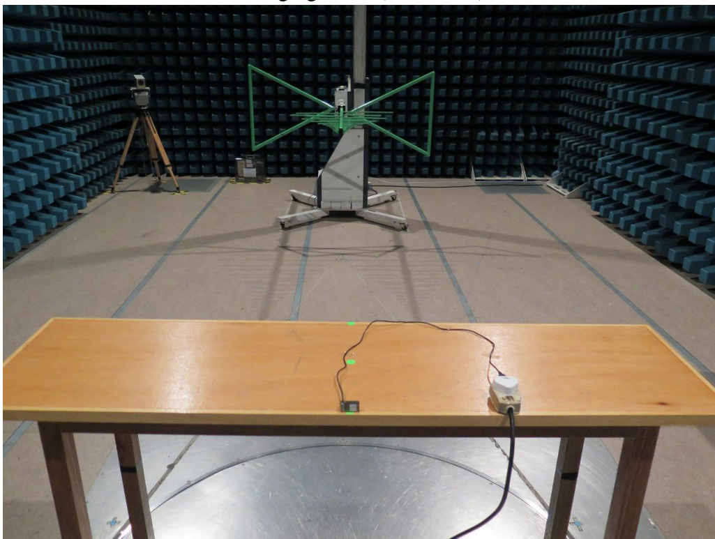
Charging mode (rear view)
