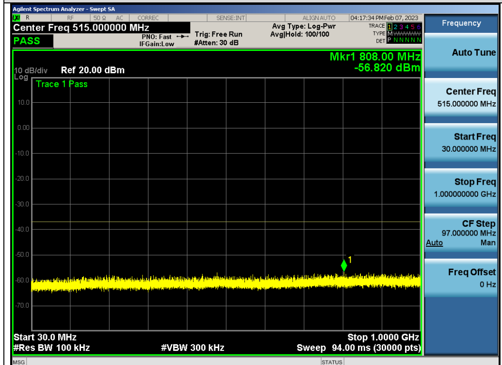
Test_Graph_802.11n40_ANT1_5310_MCS0_Frequency Band 1
