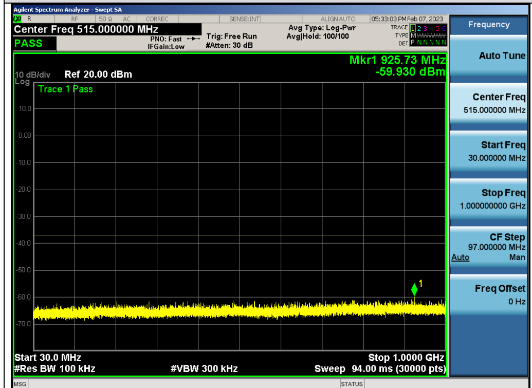
Test_Graph_802.11ac80_ANT1_5530_MCS0_Frequency Band 1
