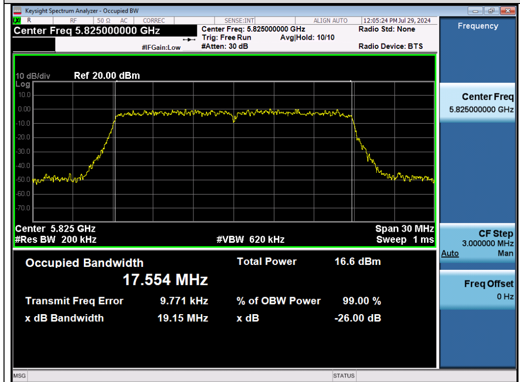
Test_Graph_802.11n20_Chain A_5825_MCS0_OBW
