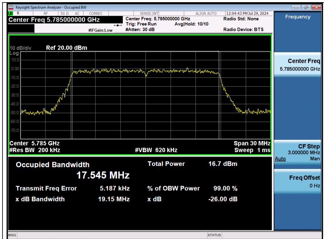
Test_Graph_802.11n20_Chain A_5785_MCS0_OBW
