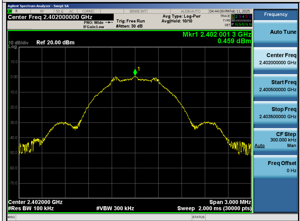
Test_Graph_SRD_2.4G_Chain B_2402_Reference Level
