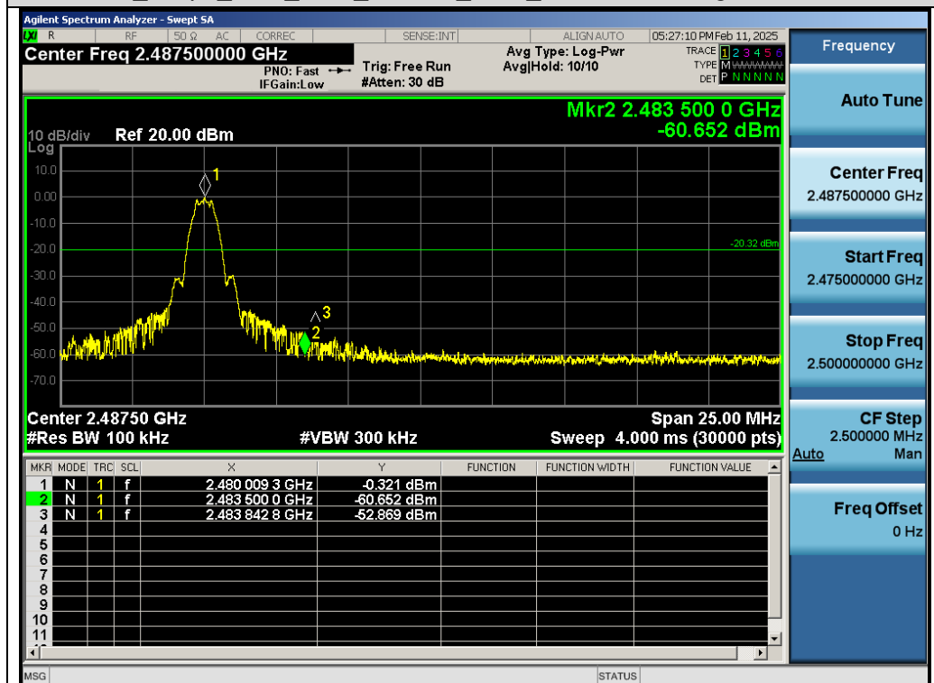
Test_Graph_SRD_2.4G_Chain A_2480_Higher Band Edge Emissions
