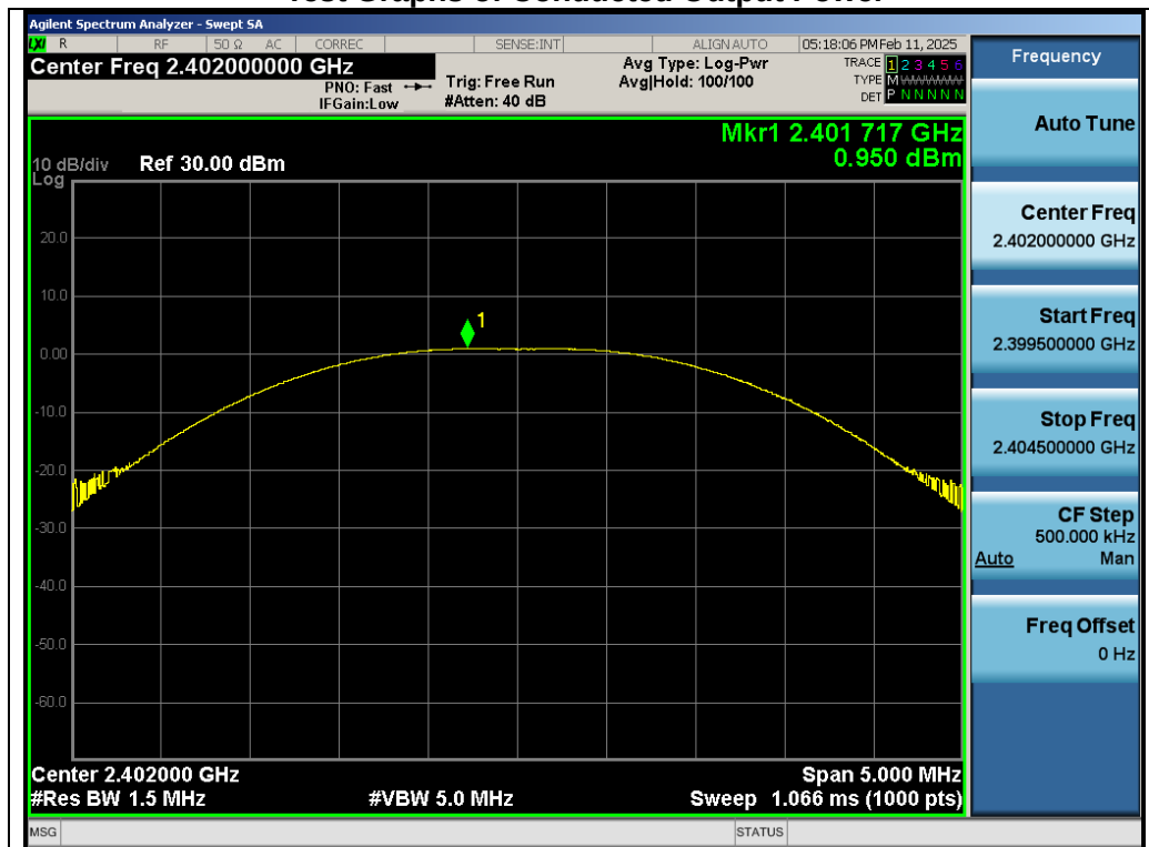
Test_Graph_SRD_2.4G_Chain A_2402_Peak Power
