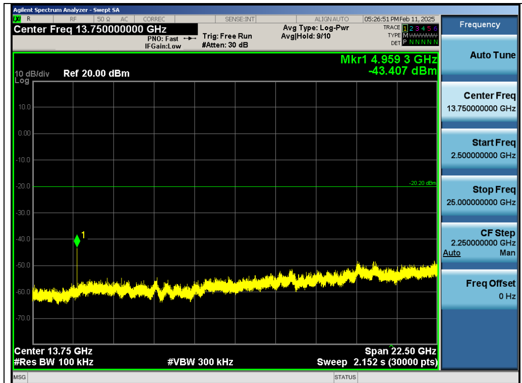
Test_Graph_SRD_2.4G_Chain A_2480_Higher Band Emissions
