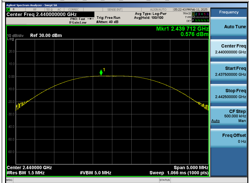
Test_Graph_SRD_2.4G_Chain A_2440_Peak Power
