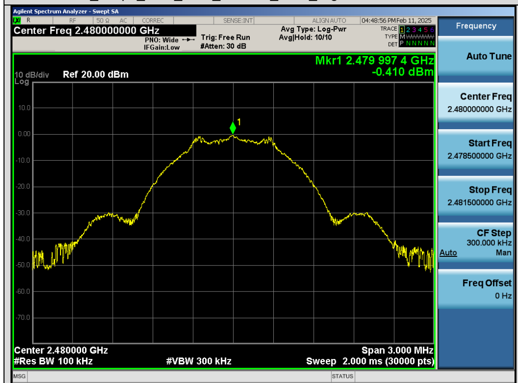
Test_Graph_SRD_2.4G_Chain B_2480_Reference Level
