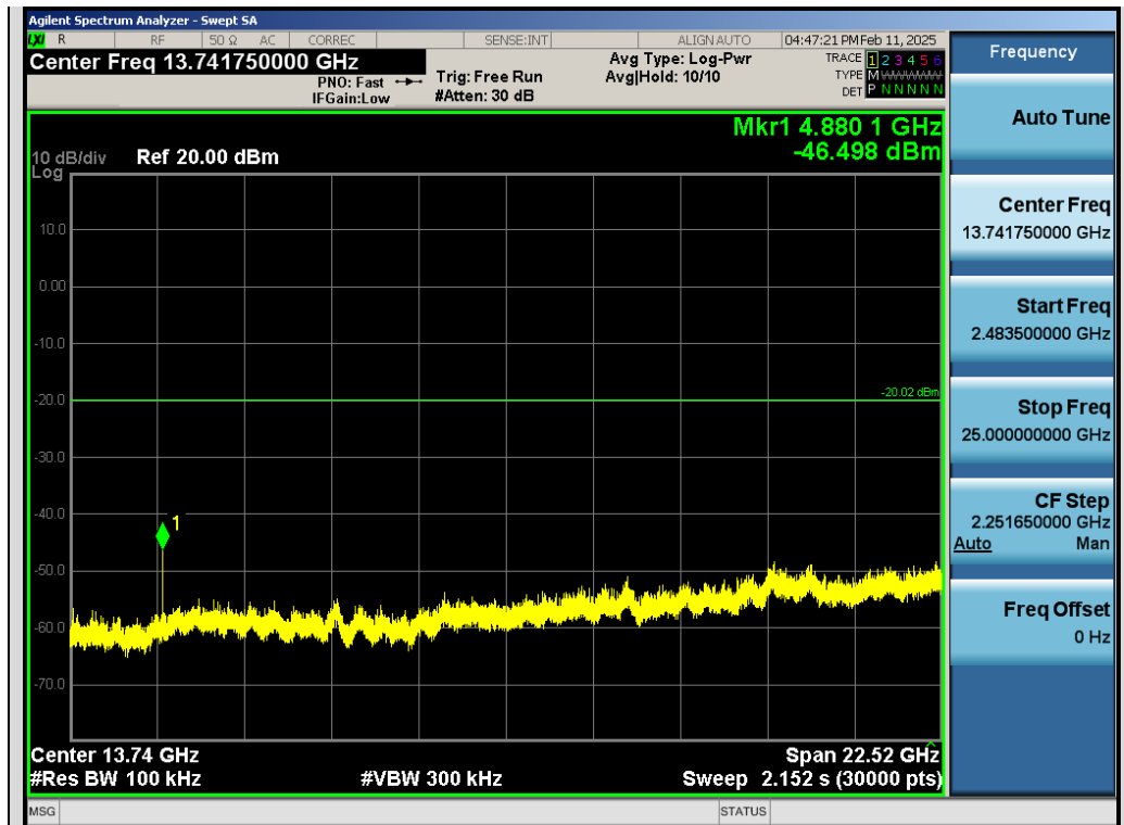
Test_Graph_SRD_2.4G_Chain B_2440_Higher Band Emissions
