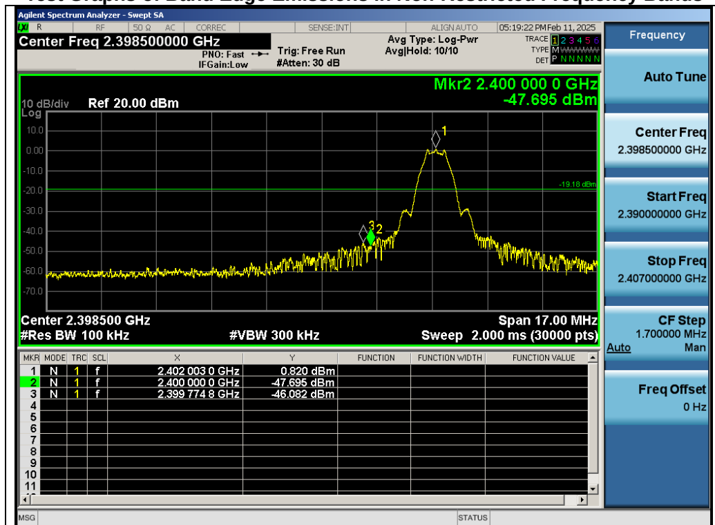
Test_Graph_SRD_2.4G_Chain A_2402_Lower Band Edge Emissions
