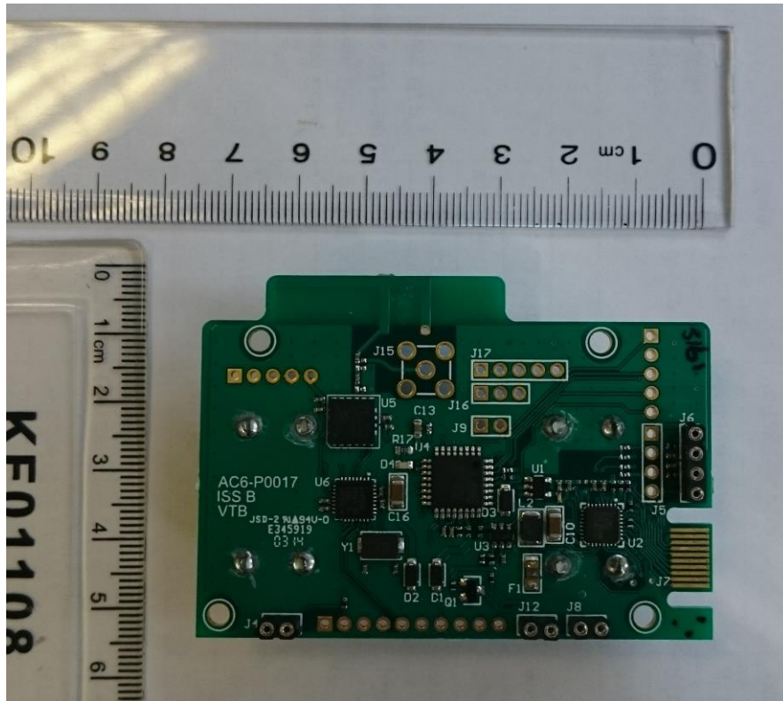
Case Open – PCB battery side
