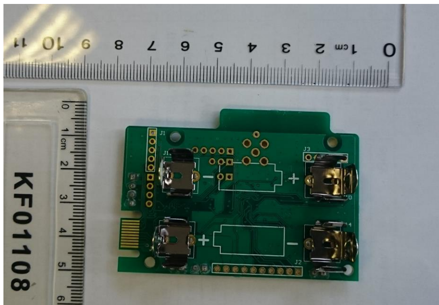
Case Open – PCB battery side
