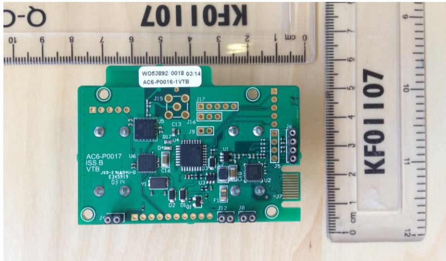
Case Open – PCB battery side
