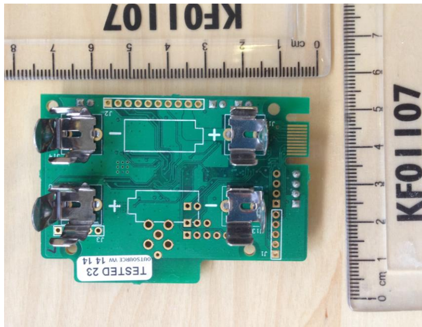
Case Open – PCB battery side
