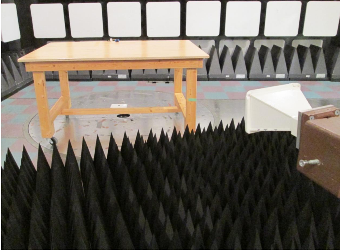
Radiated Emissions Photo 3
