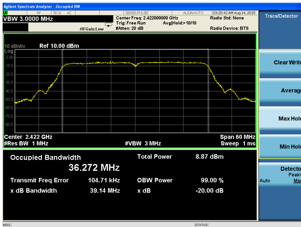
802.11n HT40 channel, 20dB bandwidth
