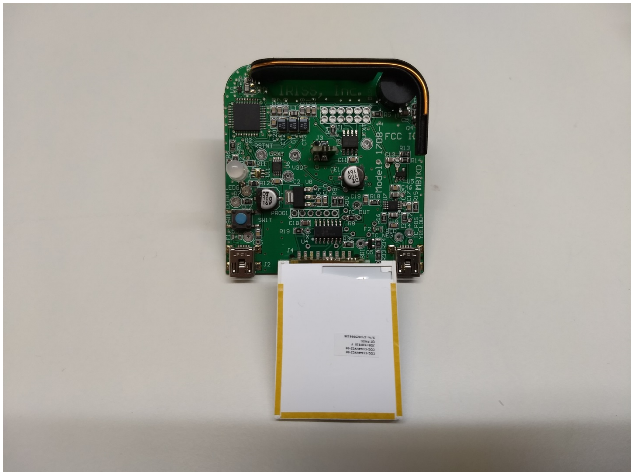
Board – Front
