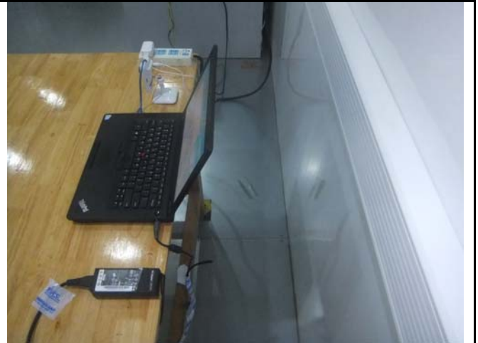
Conducted Emission and Adapter 1– Rear View
