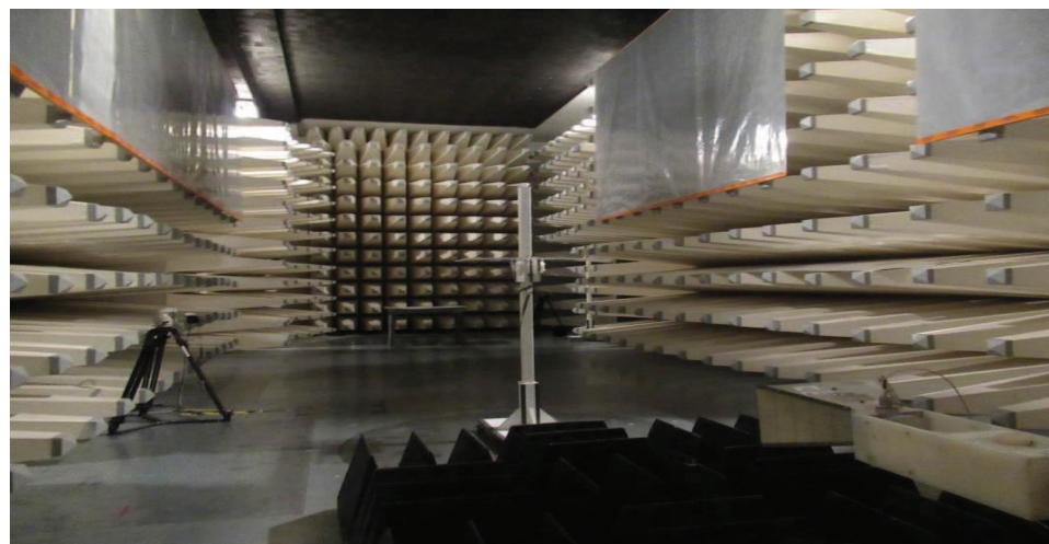
Set-up for Radiated Emission
