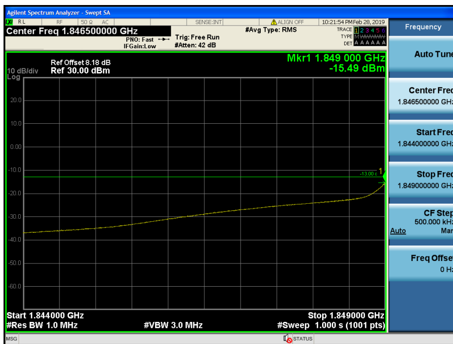
LTE Band 2 / 5MHz / 16QAM Size/Offset (25/0)
