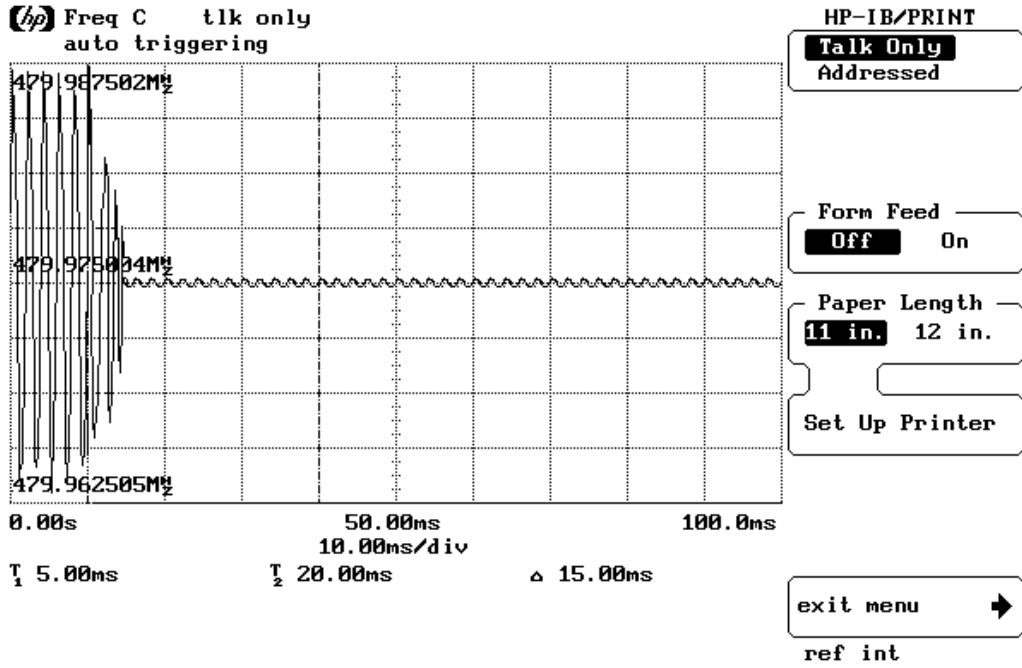
Transmitter Frequency Behavior @ 12.5 KHz Channel Separation--On to Off
