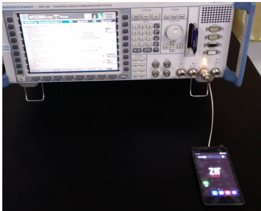
Photograph –2G&3G Conducted Test Setup
