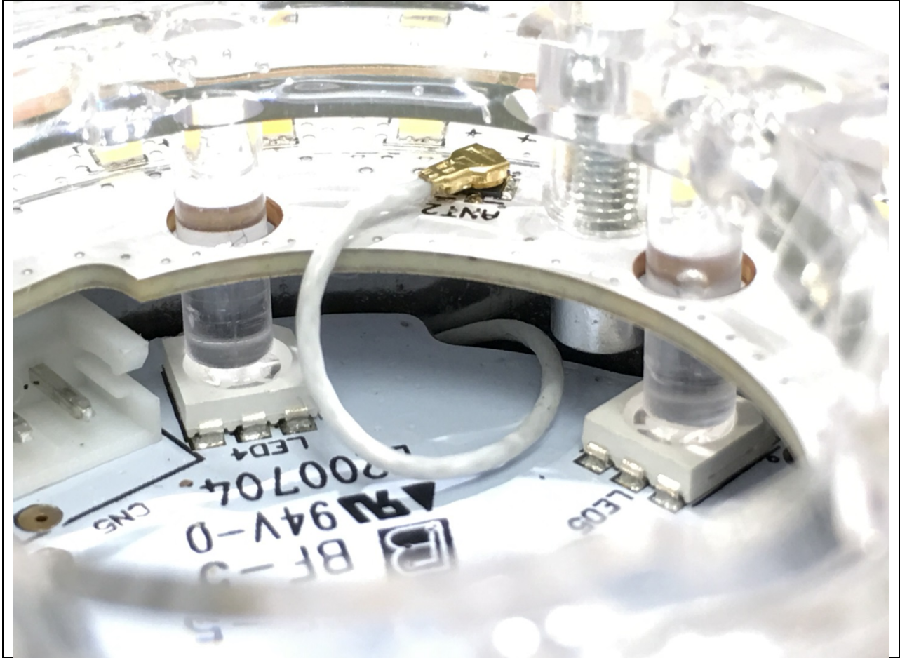
BLE RF connector to ANT2 of LED Board (from BLE Board ANT1)
