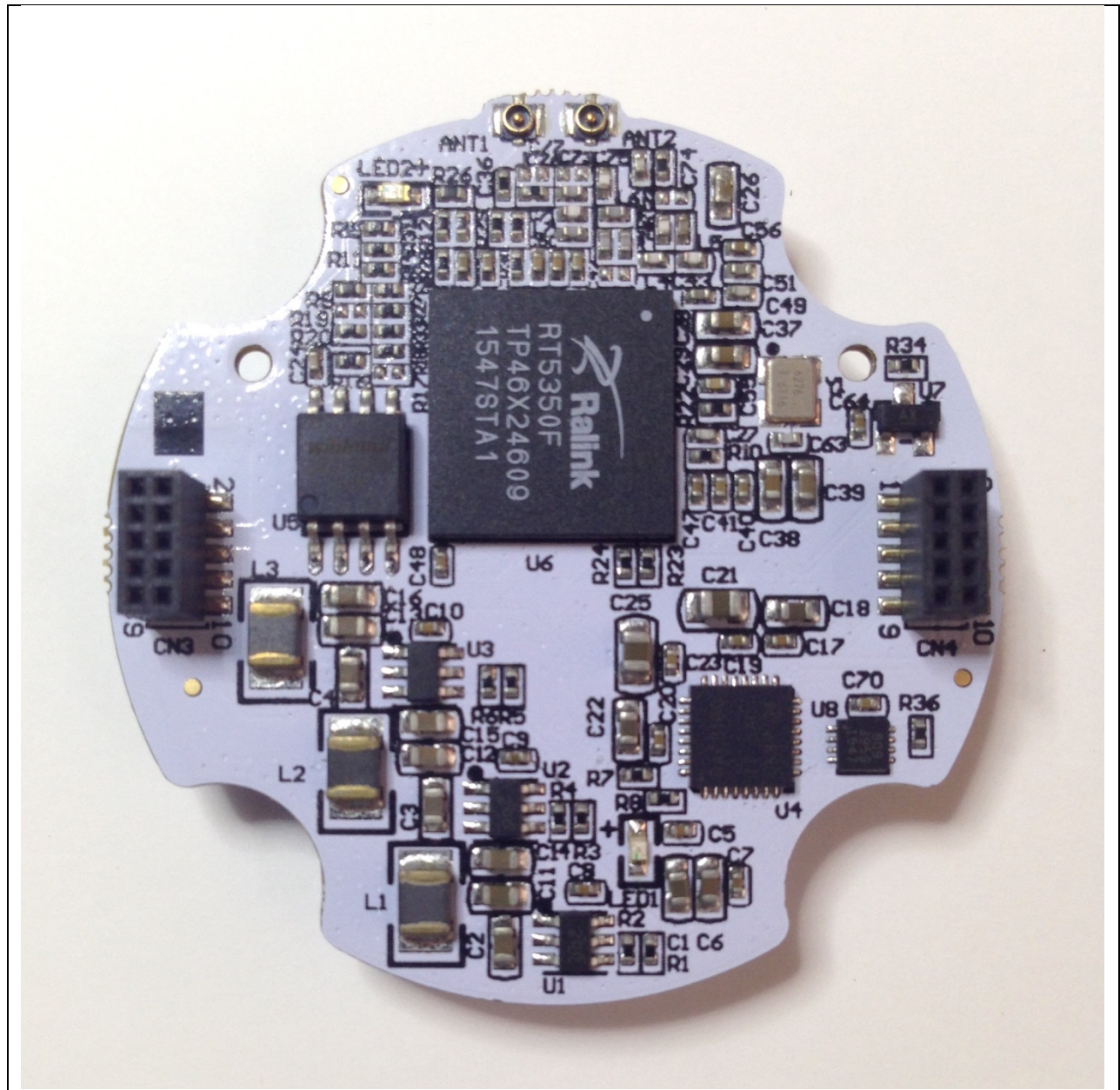
WiFi Board Top
